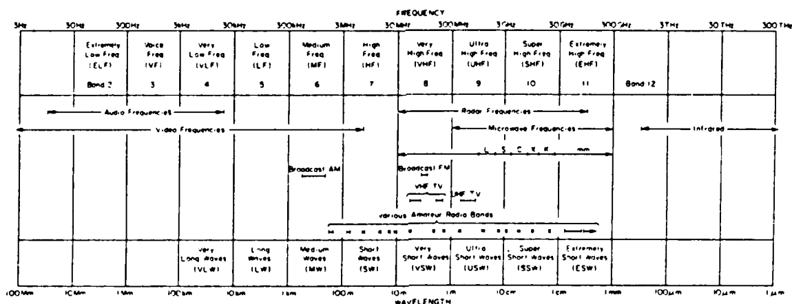
Figure 1.1. Frequency Spectrum
