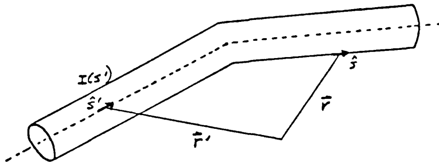
Figure 2.2. Thin-Wire Approximation Coordinate System
