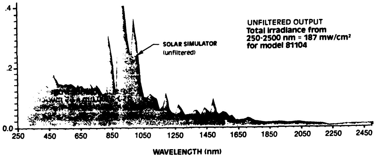
Figure 8. Unfiltered Irradiance Output from Oriel Solar Simulator
