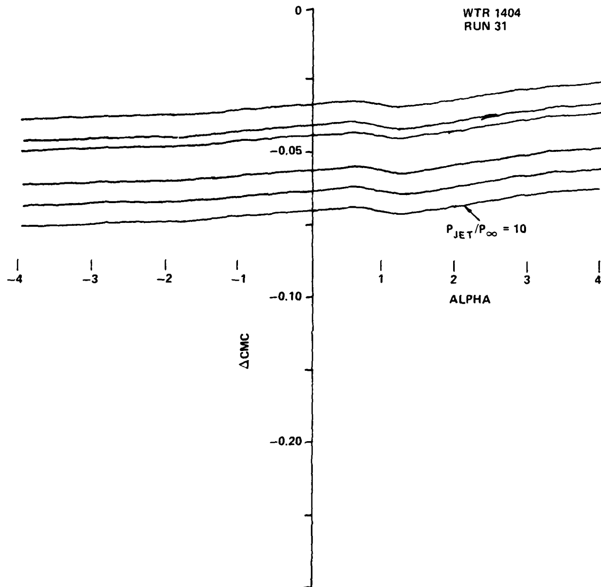
FIGURE 11b. (CONT.) PITCHING MOMENT COEFFICIENT DUE TO CONTROL EXTENSION OF 1 IN.
