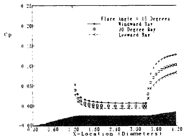
Figure 12. Pressure coefficient distribution for cone-cylinder-flare for 15° flare.
