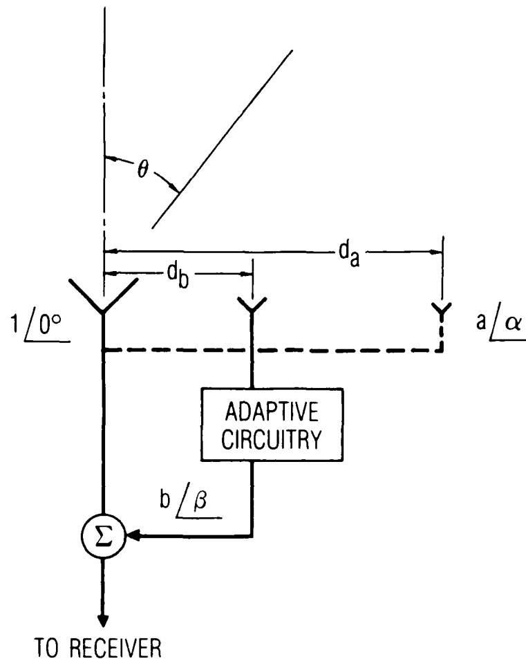
Fig. 3. Adaptive Antenna Model with Low-Level Component
