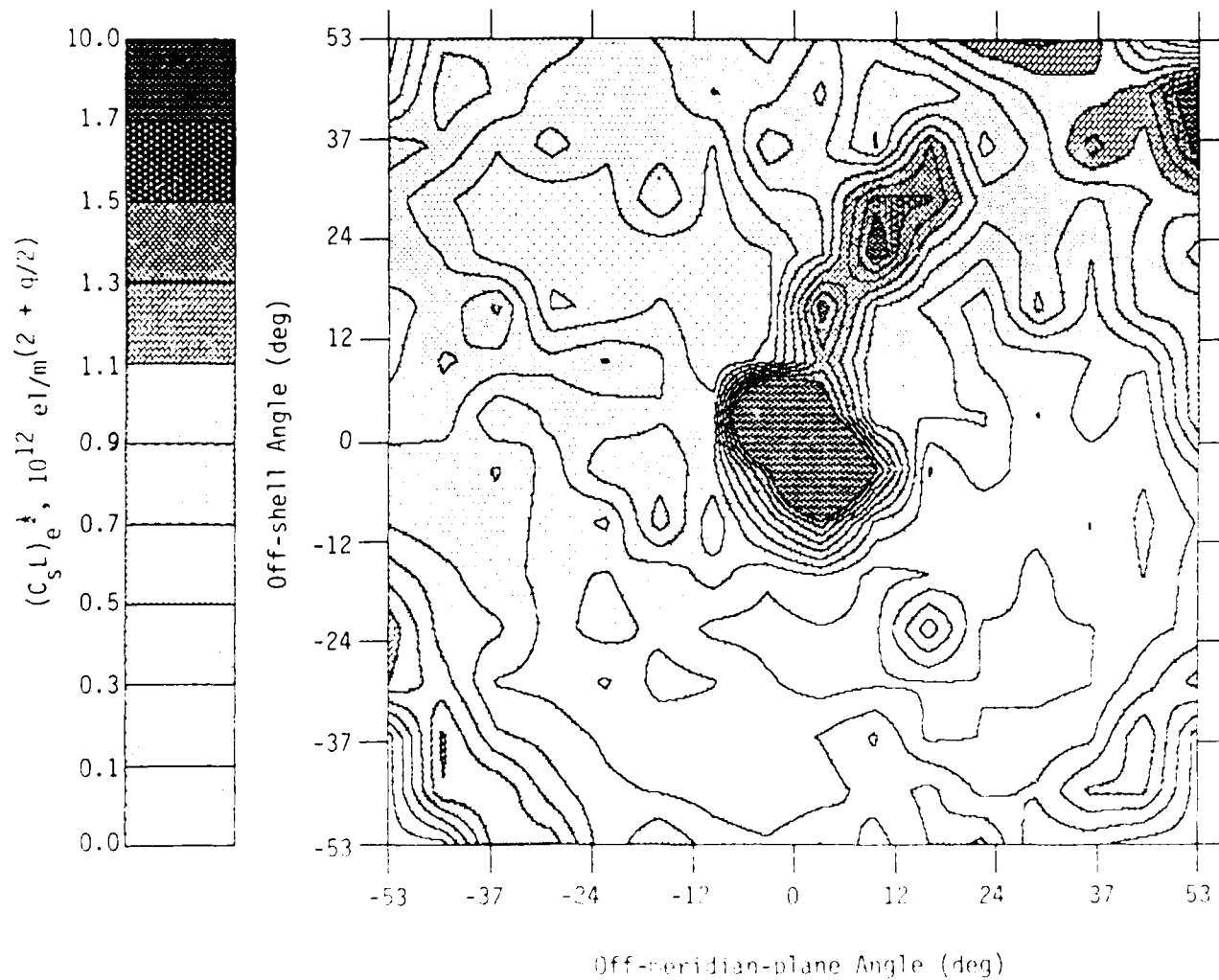
Figure 6. The two-view scan around 10 hours magnetic local time, which displays the three-part structure of field-aligned anisotropy.
