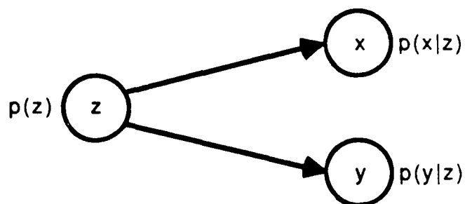
Figure 2.1 x and y Conditionally Independent Given z
