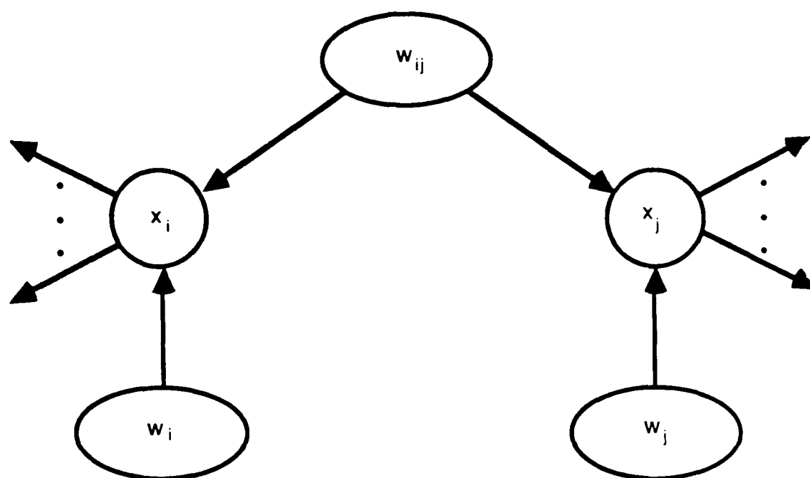
Figure 3.1 Conditional Independence
