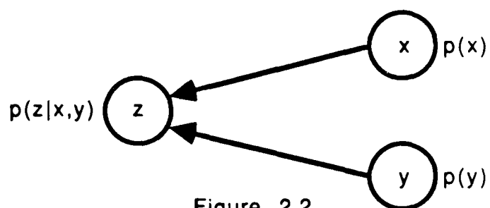
Figure 2.2 x and y Independent
