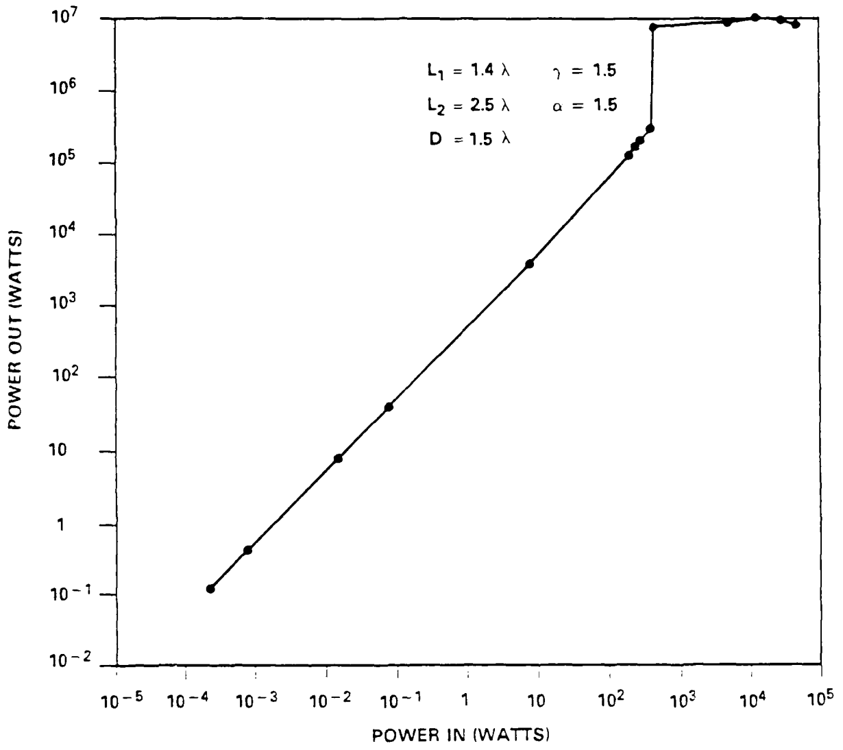
Figure 6. Theoretical Drive Curve for a Two-Cavity, Phase-Locked Gyrokystron Amplifier. L_1 and L_2 refer to the cavity lengths, D is the drift length between the two cavities, and \gamma is the relativistic factor.
