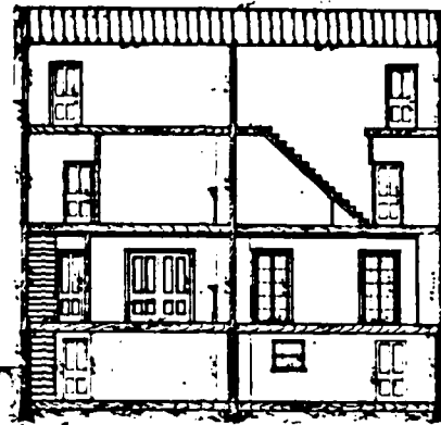
SECTION - LINE A-B
