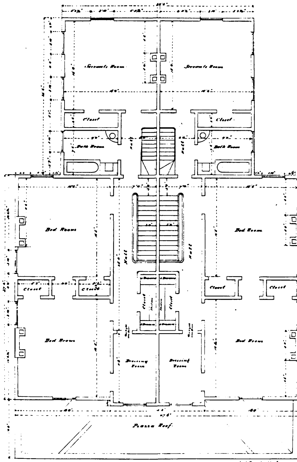
SECOND FLOOR.
