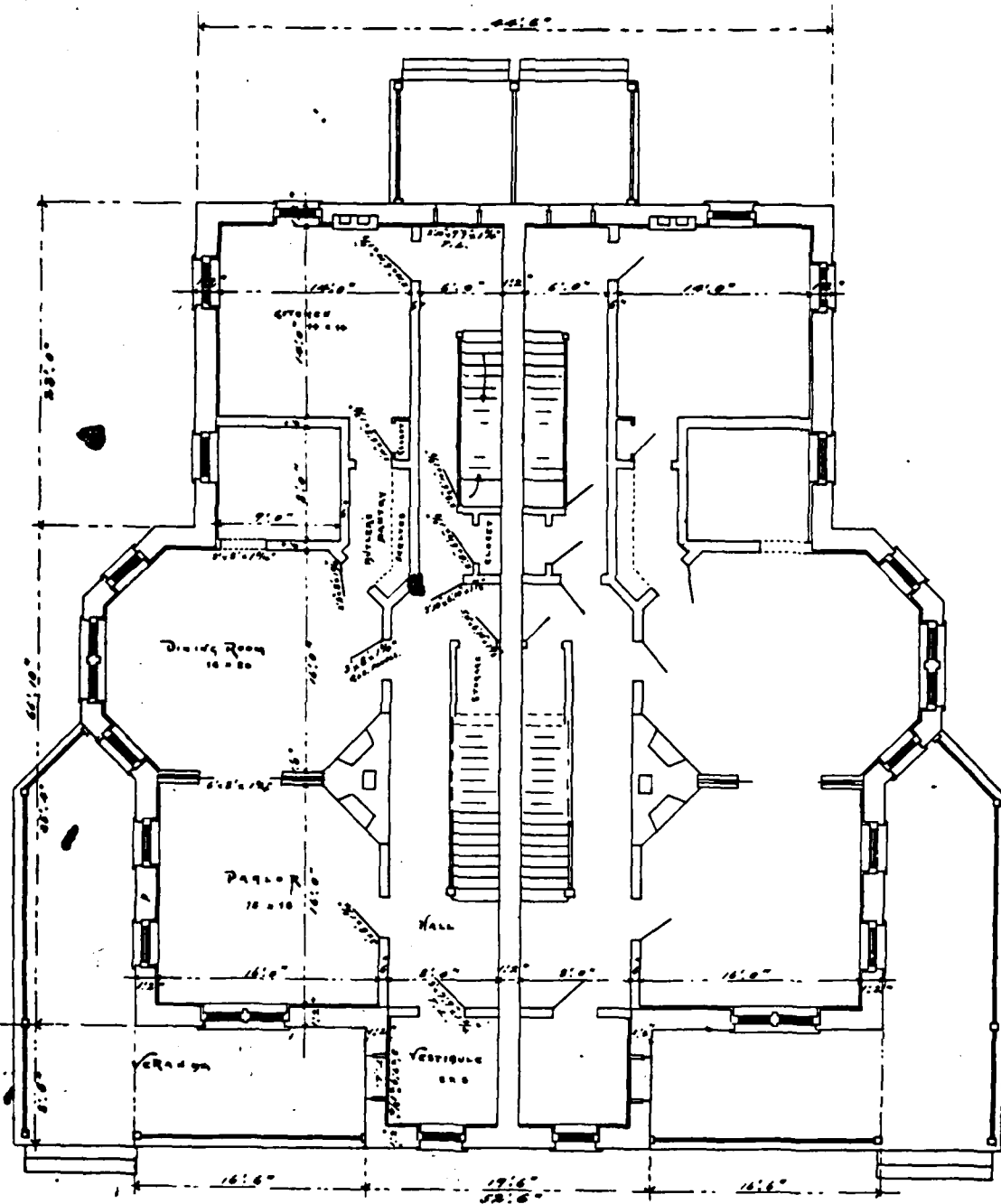
FIRST FLOOR PLAN - CEILING 10'-0"
