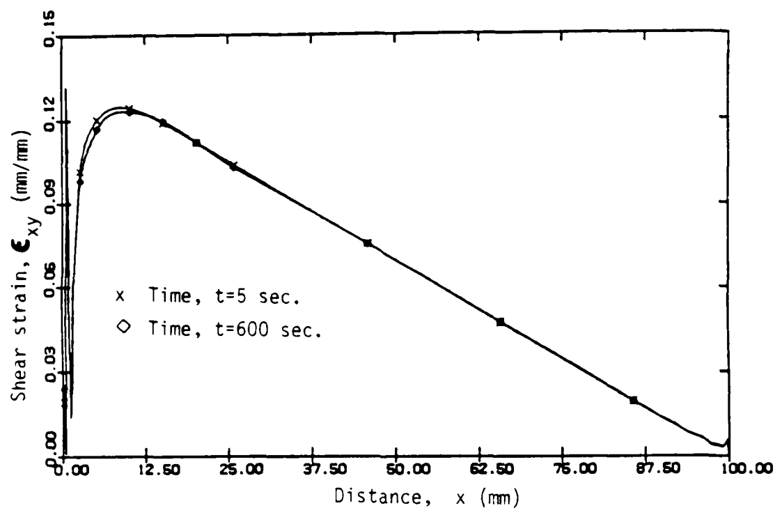
(a) Shear strain in aluminum at y=4.96 mm
