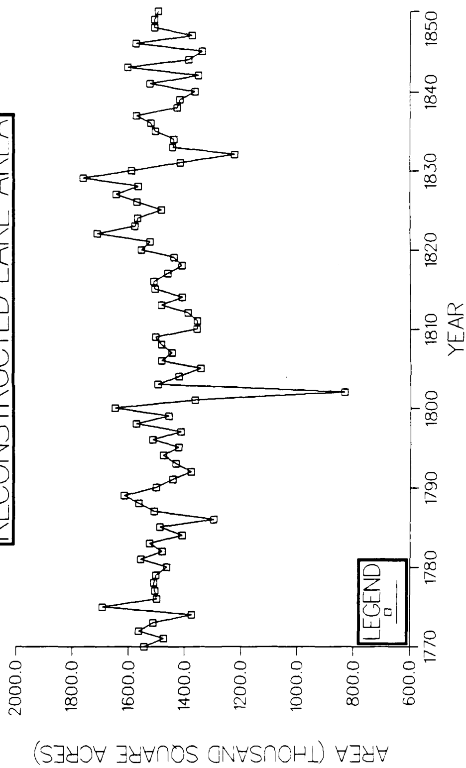
Figure 7. Reconstructed lake level (1770 - 1850).
