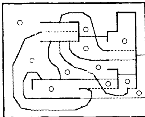
Figure 4. The adjacency graph of the sketch in Figure 1. Dashed lines are hurdles, and circles are nodes of the adjacency graph. Wherever two such nodes are adjacent across a wire or hurdle, there is a "wire edge" or "hurdle edge", respectively, in the adjacency graph. These edges are omitted for clarity. Adjacency across features is not represented in the adjacency graph.
