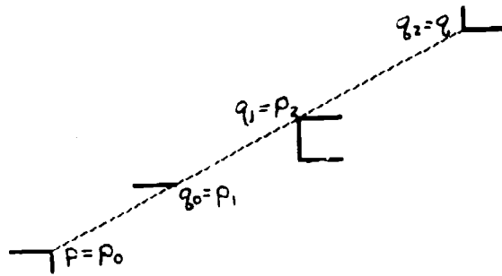
Figure 8. The line segment s_\lambda = \psi(b_\lambda) just as it ceases to be a cut.
