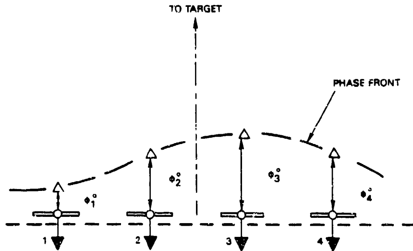
FIGURE 4. Four-Element Antenna Array With Impinging Wave. A sample locus of constant phase is shown. The \phi_1 represent the electrical distance 2\pi z_1/\lambda to the constant phase locus, where z_1 is the physical distance.
