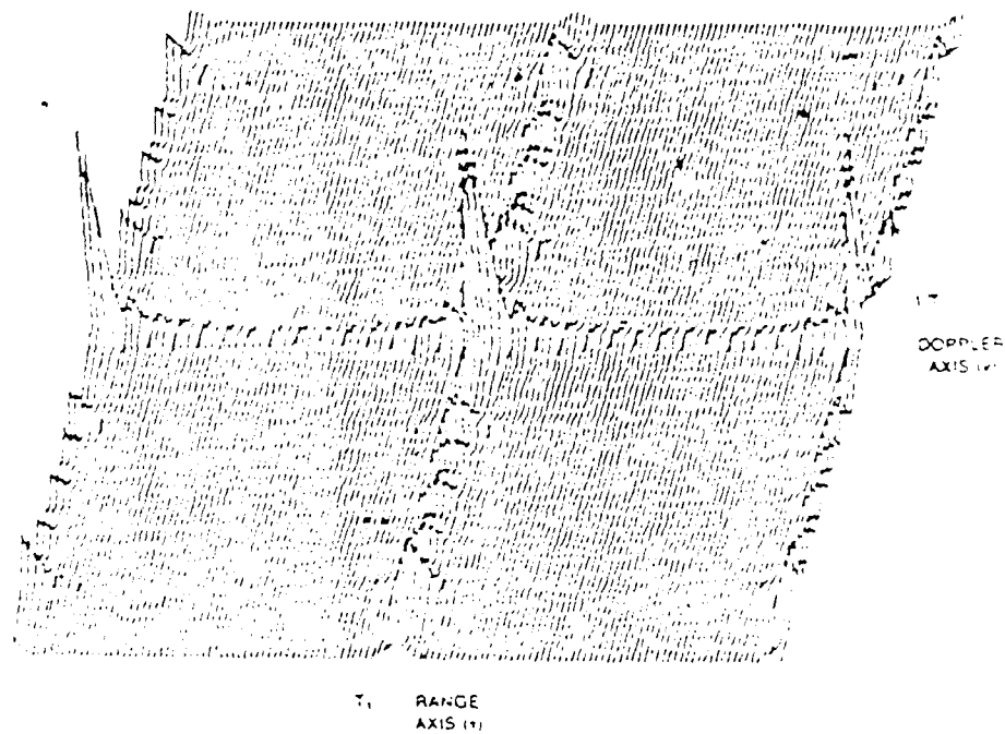
Square root of ambiguity surface for 16 pulse train (15 bit missequence code)
