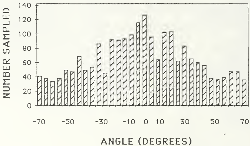
Figure 3.4. Slope histogram of the bottom surface of a roughened acrylic plate used to model an Arctic rubble field.
