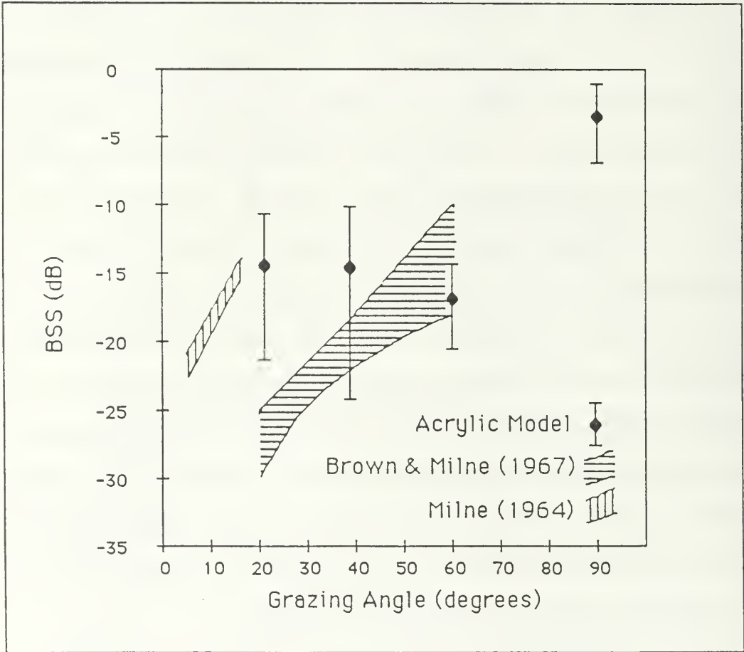
Figure 6.20: Backscattering strength as a function of grazing angle for the acrylic model of a rubble field compared with actual Arctic backscatter from rough ice.
