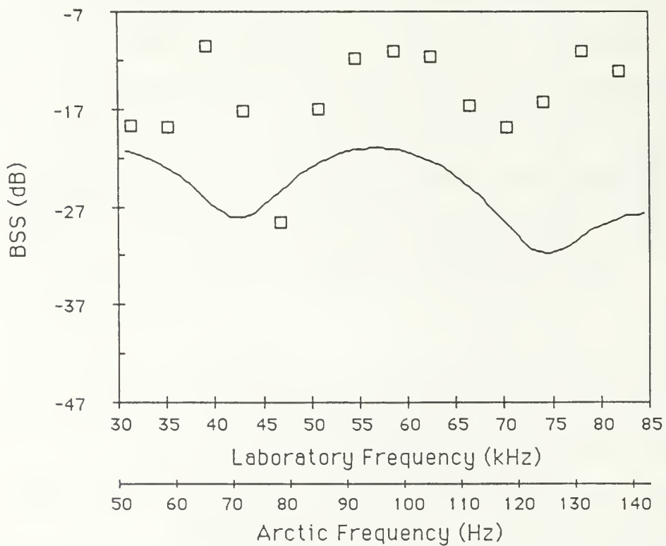
Figure 6.15: Temporal and spectral backscatter from the model of a ridge keel. The squares are measured backscattering strength, lines are the calculated BSS using Biot-Tolstoy diffraction theory. The grazing angle is 29^\circ .
