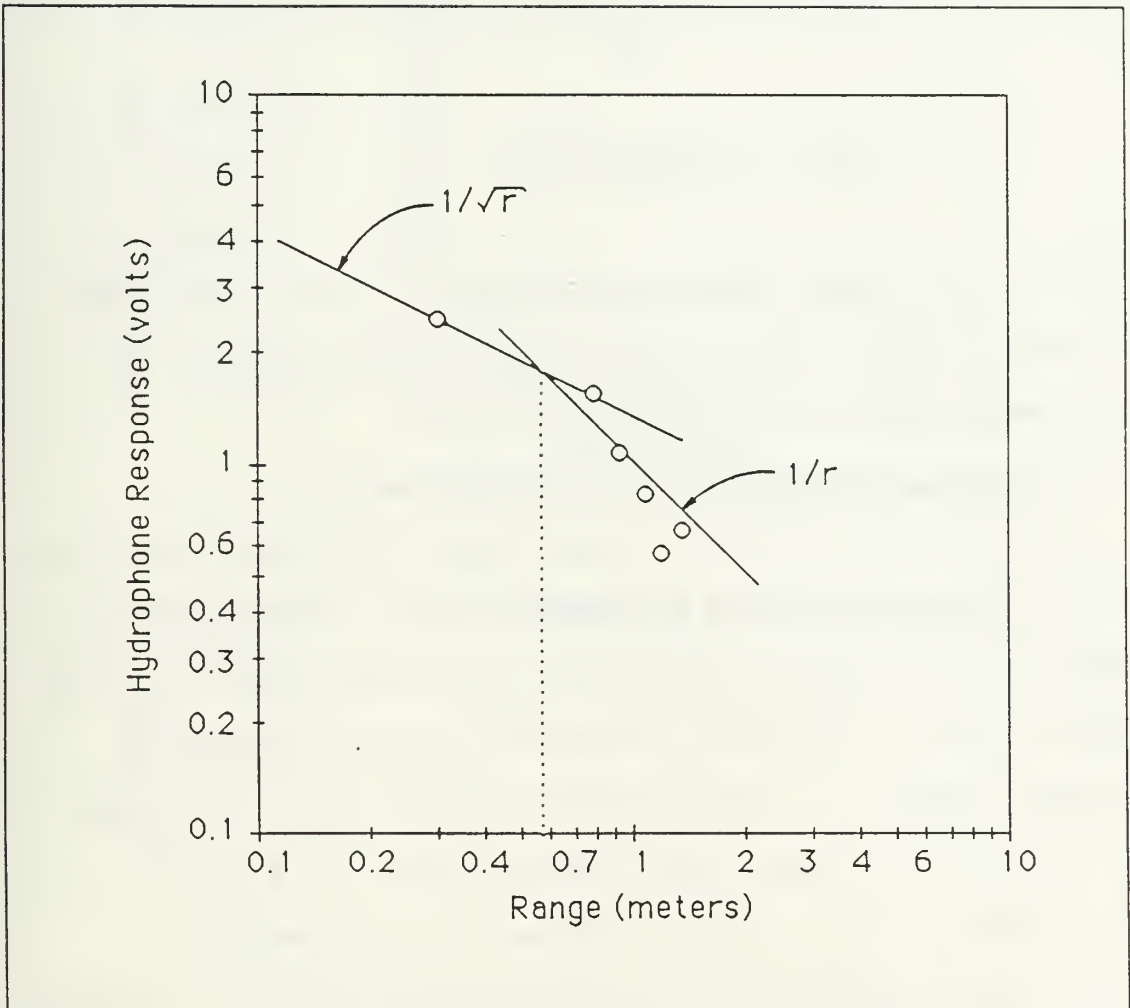
Figure 6.4: Results of the measurements using the geometry shown in Figure 6.3, where the range is r . Data indicates that the geometrical divergence is cylindrical ( \propto 1/\sqrt{r} ) at short range and spherical ( \propto 1/r ) at longer ranges.
