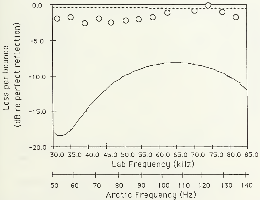
Figure 5.5, Temporal and spectral forward scatter from the laboratory wedge. Solid line is theoretical rigid wedge diffraction from the wedge keel. Dashed line is the theoretical combination of B-T diffraction and M&M reflection. Circles are experimental results. Grazing angle is 33 degrees.
