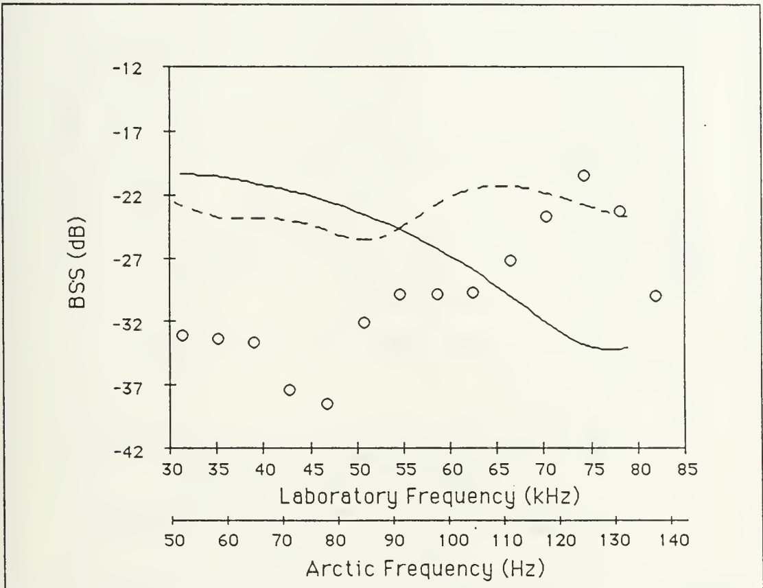
Figure 6.10: Spectral backscatter from an open lead with width 1 cm (6 m in the Arctic). Solid line from diffraction theory for two visible edges and one surface reflection. Dashed line is diffraction theory plus the effect of multiple reflections in the lead. Points are measured values. Grazing angle is 15^\circ .
