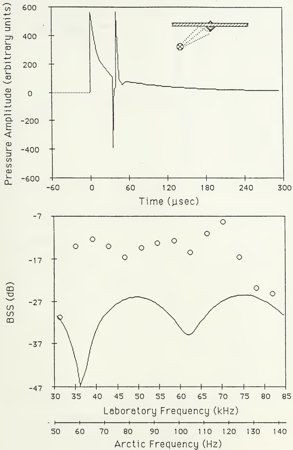
Figure 6.15: Temporal and spectral backscatter from the model of the ridge keel. The circles are measured back-scattering strength, lines are the calculated BSS using Biot-Tolstoy diffraction theory. The grazing angle is 15^\circ .
