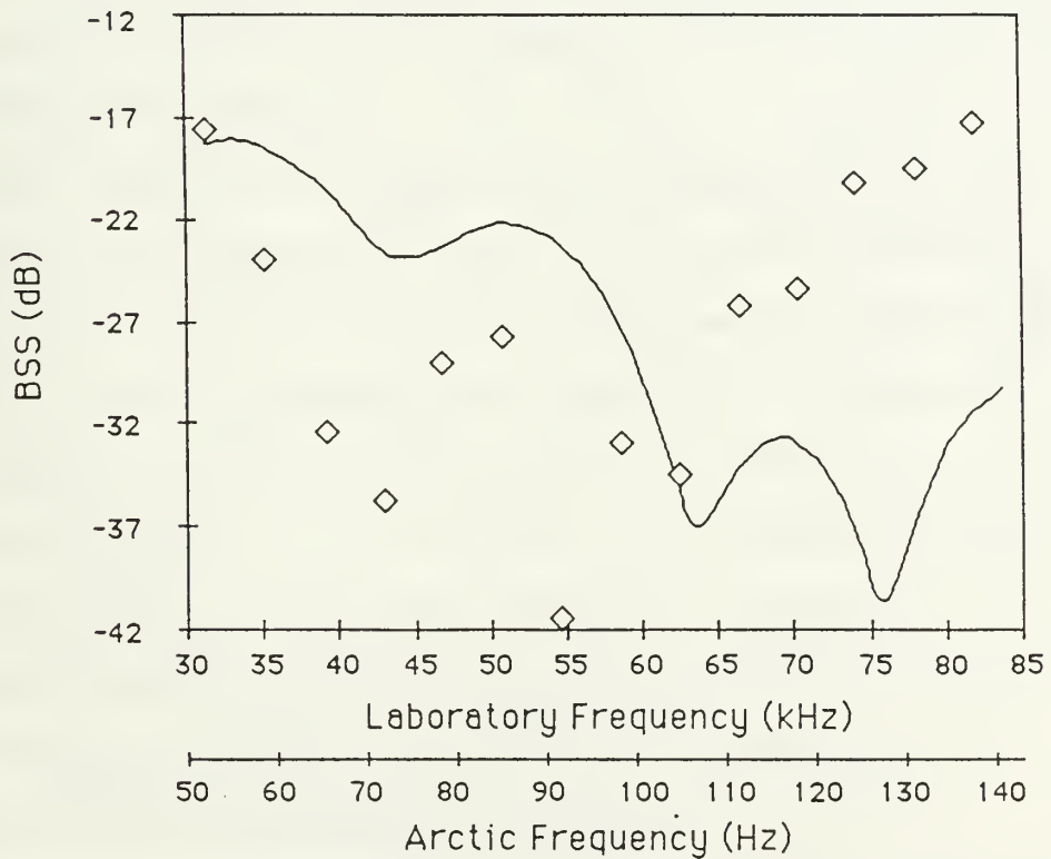
Figure 6.17: Temporal and spectral backscatter from the model of a ridge keel. The diamonds are measured backscattering strength, lines are the calculated BSS using Biot-Tolstoy diffraction theory. The grazing angle is 47^\circ .
