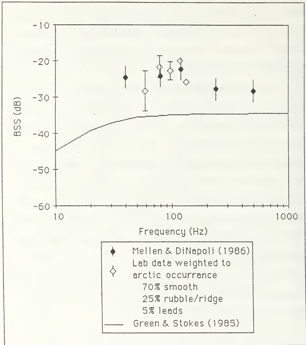
Figure 6.2.1: Composite BSS computed for the acrylic model of the Arctic ice scaled to arctic frequencies plotted along with Arctic measurements of BSS. Curve is from a computer model of arctic backscatter which does not consider mode conversion.
