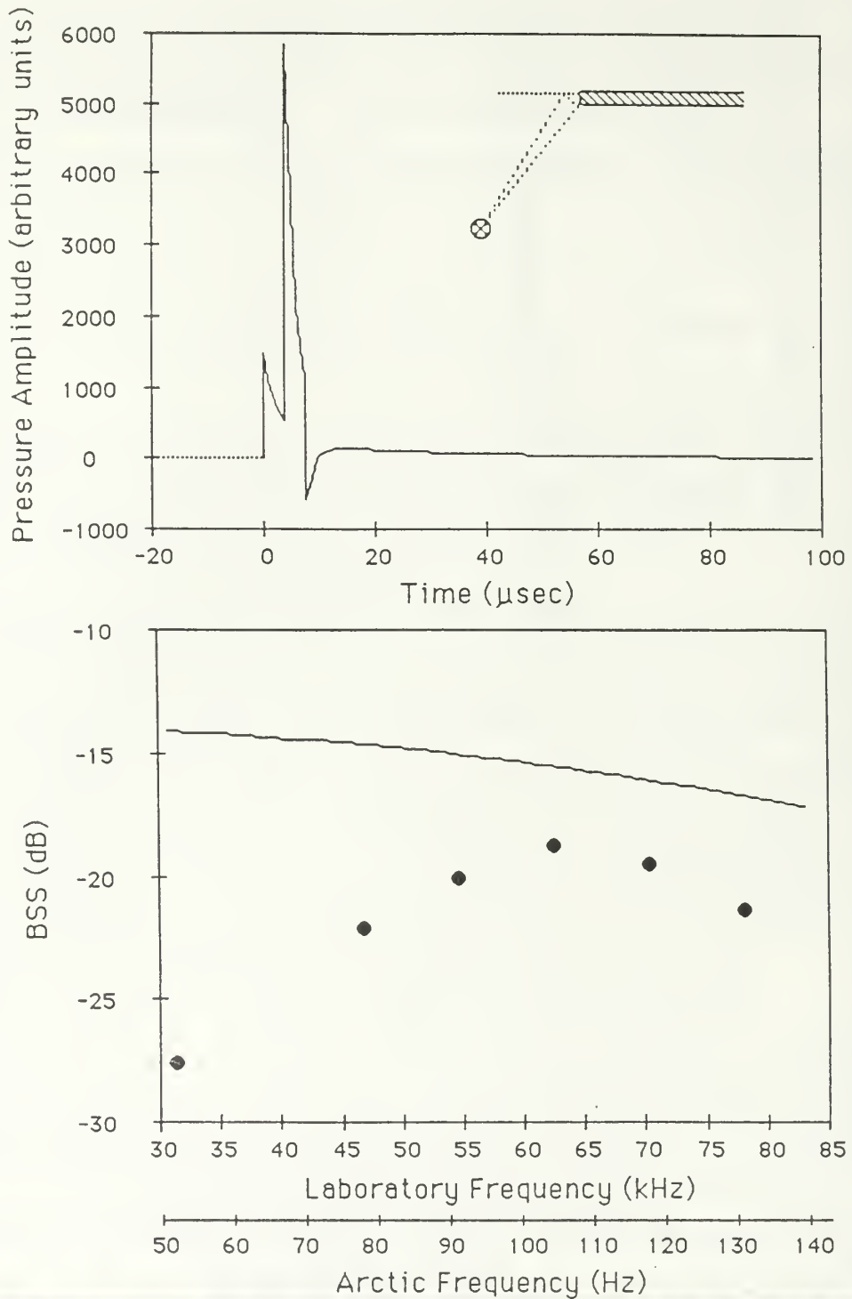
Figure 6.5: Temporal and spectral backscatter from the leading edge of the acrylic plate. Solid line is theoretical rigid wedge diffraction from the submerged edge and its surface reflection. The circles are the experimental data. Grazing angle is 45^\circ .
