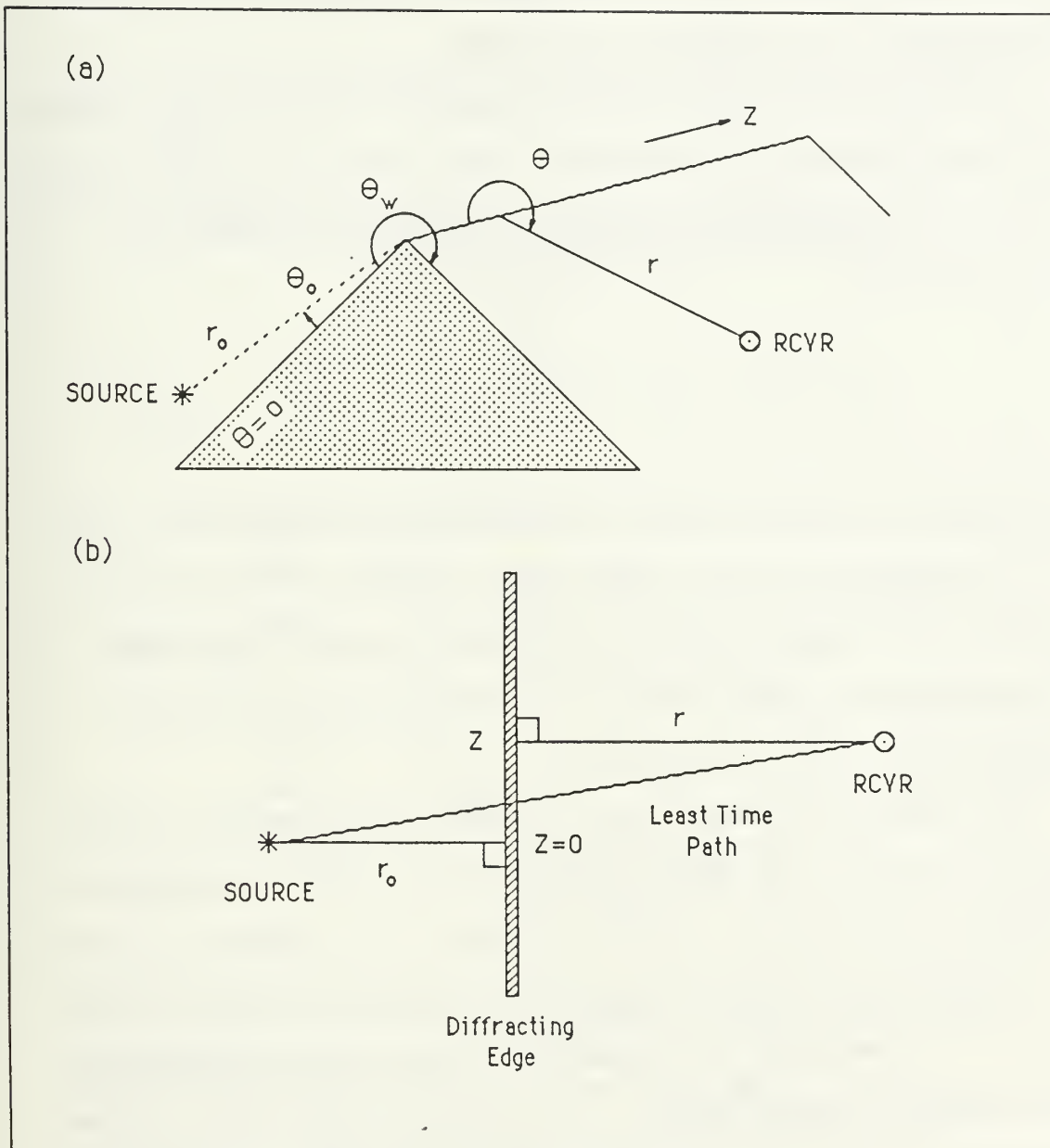
Figure 4.1: (a) Wedge geometry for equations 4-1 thru 4-3. (b) Unfolded geometry.
