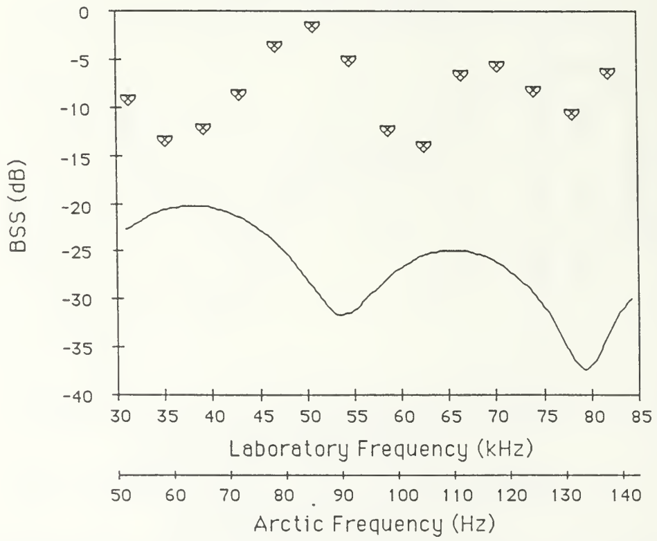
Figure 6.18: Temporal and spectral backscatter from the model of a ridge keel. The symbols are measured back-scattering strength, lines are the calculated BSS using Biot-Tolstoy diffraction theory. The grazing angle is 63^\circ .
