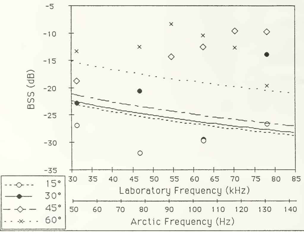
Figure 6.8: Temporal and spectral backscatter from a lagging edge of the acrylic plate. Lines are theoretical backscatter from a single edge at grazing angles of 15, 30, 45, and 60°. Points are the experimental data.
