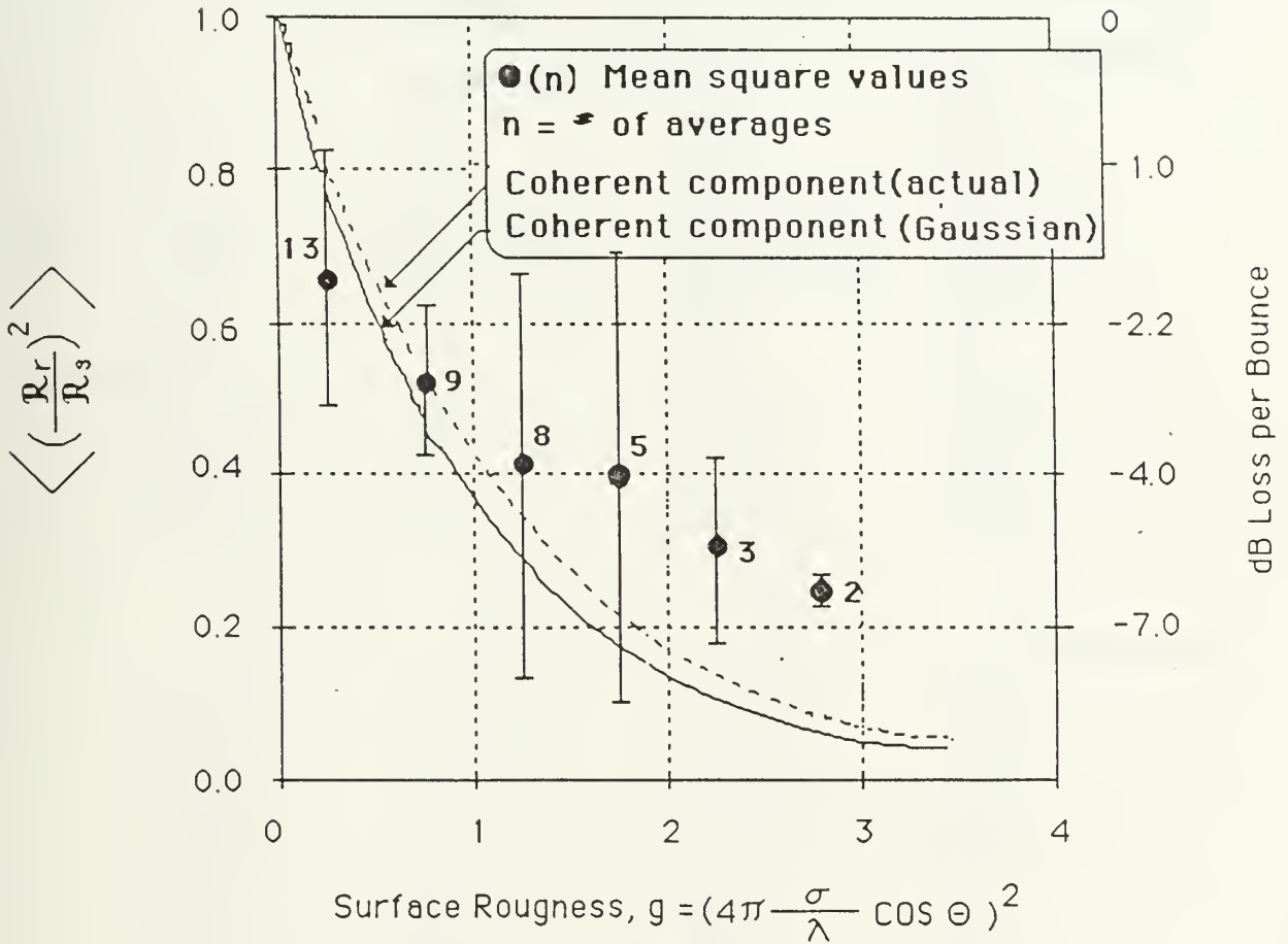
Fig. 5.4 Specular scatter at model of water-rubble ice bottom interface. Smooth curve represents the theoretical value for the coherent component of scatter from a Gaussian surface. Dashed curve represents the theoretical value for the coherent component of scatter from the measured statistical surface. In both theoretical cases, R_s is assumed 1. Dots represent mean of experimental results. Bars indicate standard deviation measured over several frequencies and angles. Boldface number indicates number of data points averaged.
