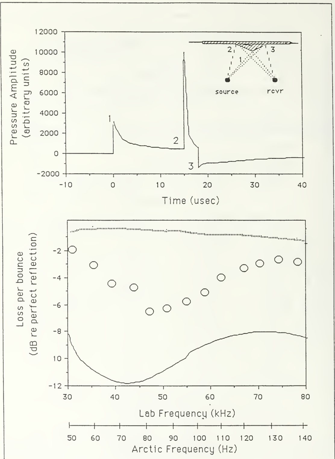
Figure 5.6. Temporal and spectral forward scatter from the laboratory wedge. Solid line is theoretical rigid wedge diffraction from the wedge keel. Dashed line is the theoretical combination of B-T diffraction and M&M reflection. Circles are experimental results. Grazing angle is 45 degrees.
