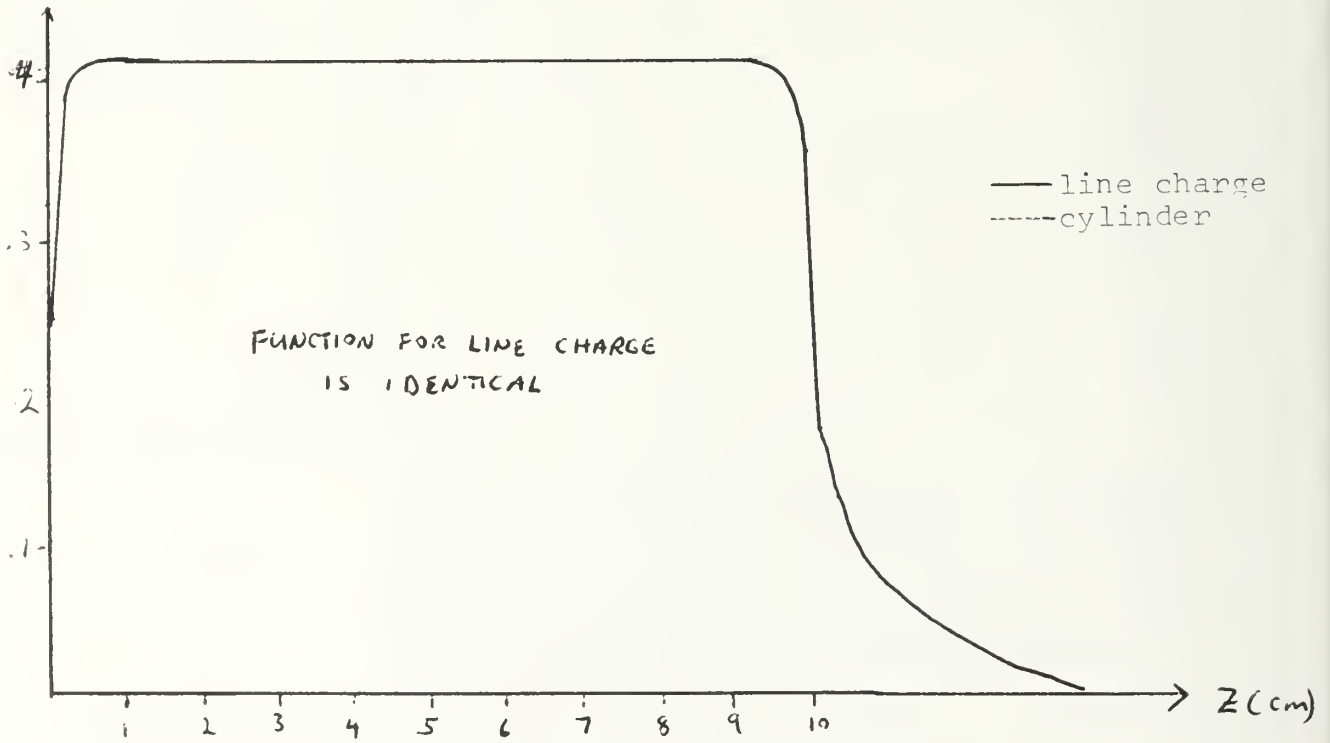
Figure 9: E ( 4\pi\epsilon/\rho ) vs Z for cylinders of various lengths a_0 = .1 \text{ cm} , b = .15 \text{ cm}
