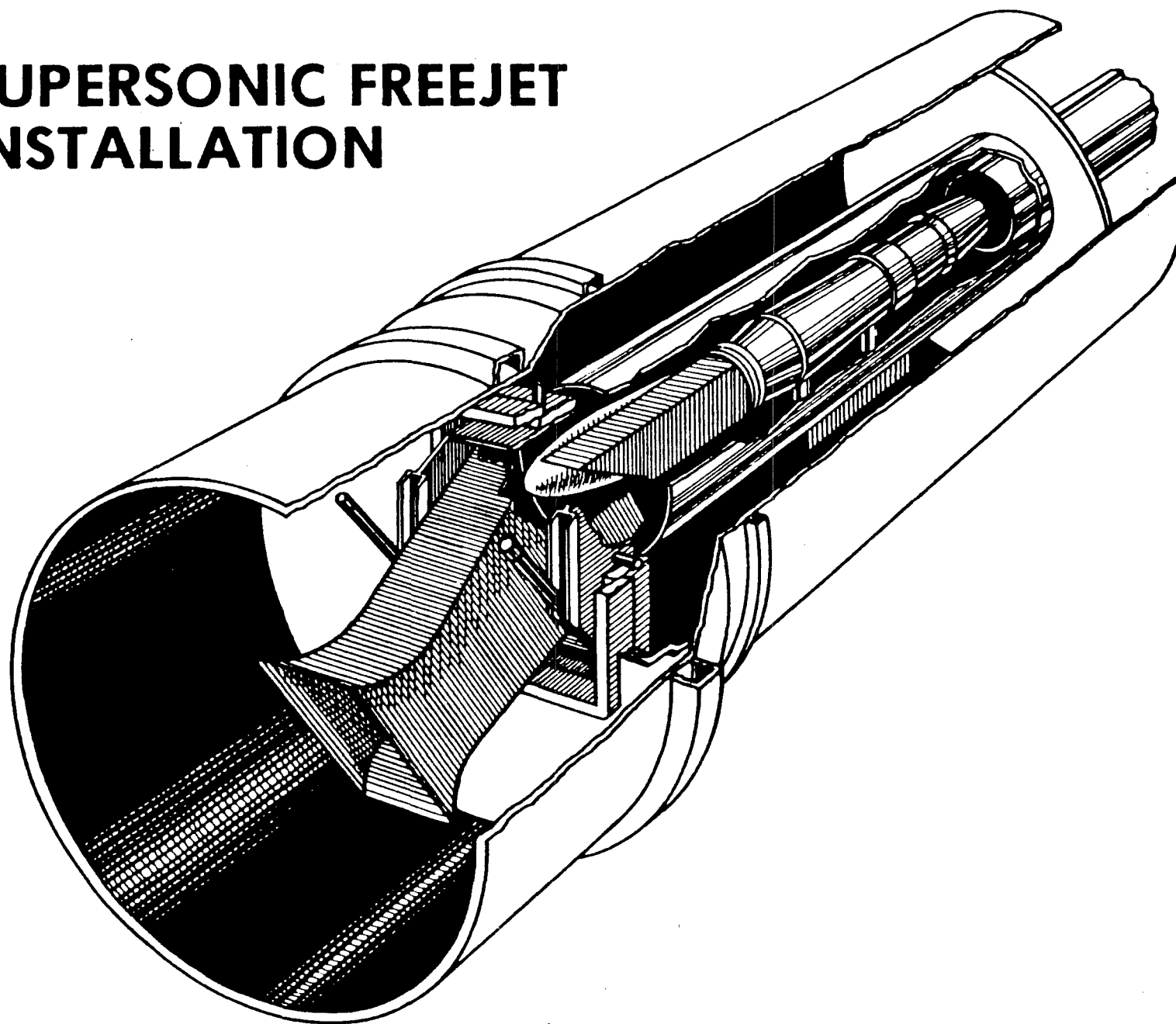
Figure 3.4 Supersonic Freejet Testing Concept for ASTF
