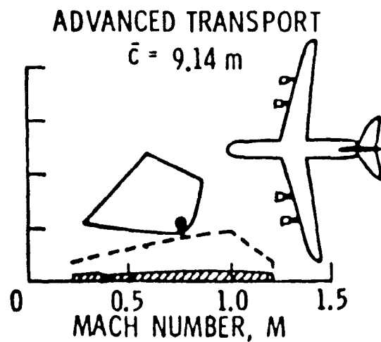
Figure 3.1 U.S. Subsonic/Transonic Wind Tunnel Capability
