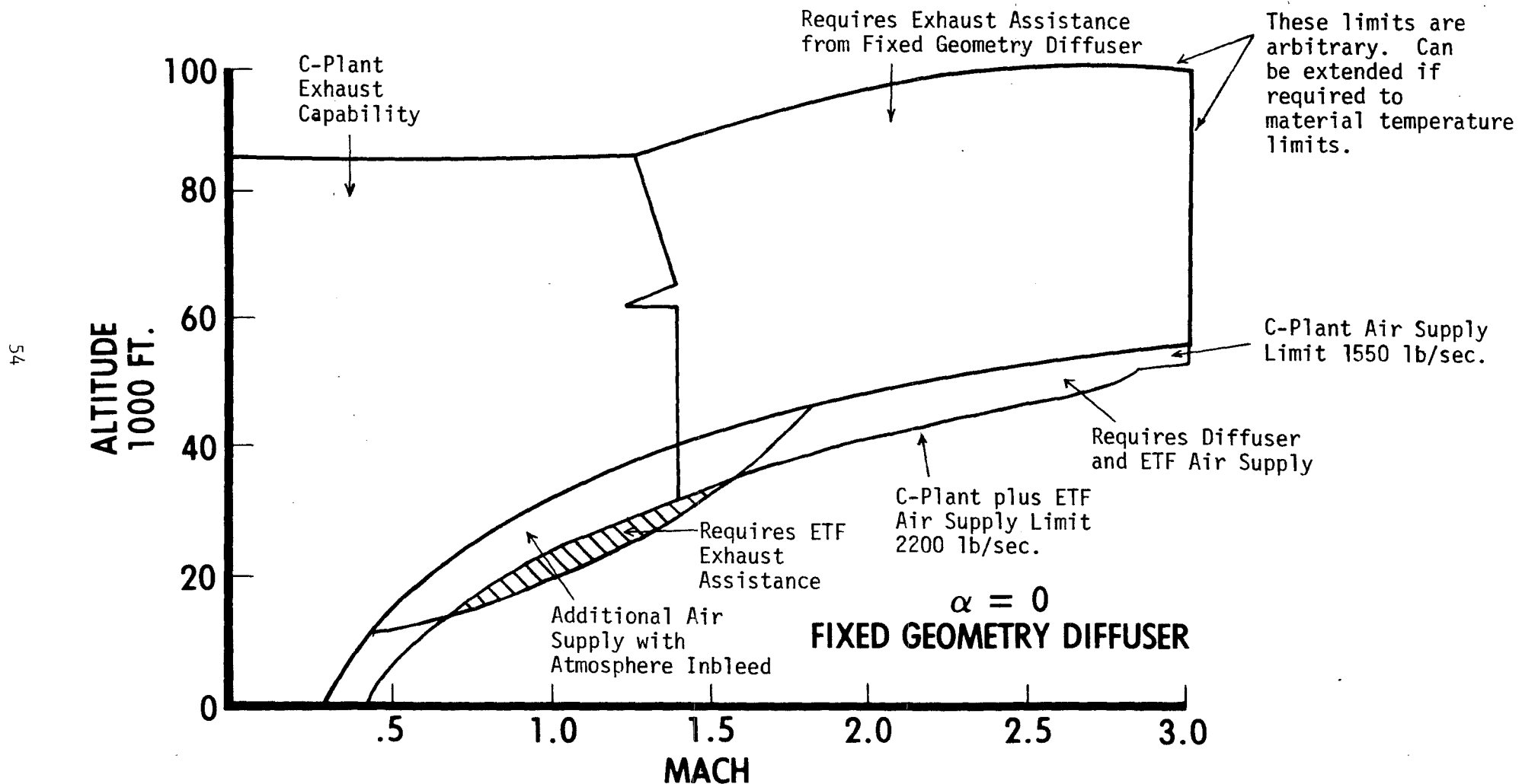
Figure 4.7 Proposed Free Jet Test Envelope for ASTF with 60 Ft 2 Nozzle
