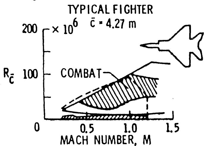
Figure 3.1 U.S. Subsonic/Transonic Wind Tunnel Capability
