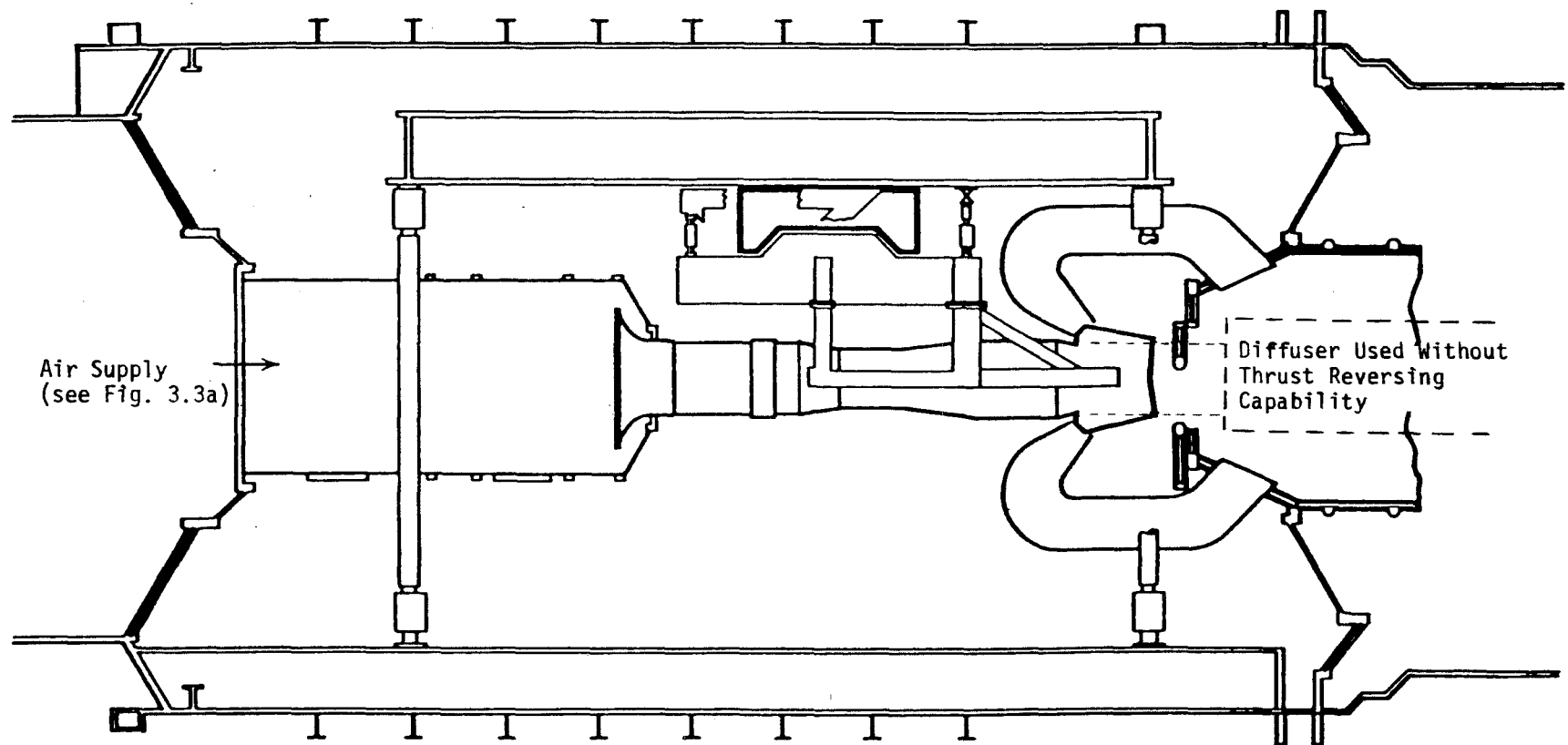
Figure 4.4 Connected Pipe Testing as Used in Engine Test Facilities
