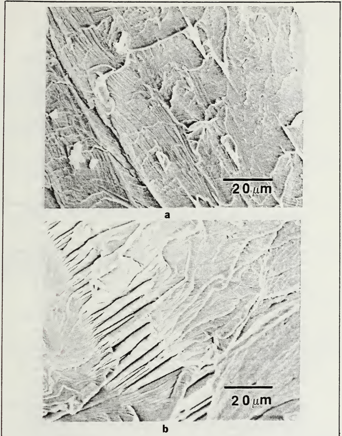
Figure A.6 Fracture Surface for Tensile Specimen of Furnace Cooled VACROSIL-010(Mo) annealed 1 hour at (a) 1000°C (1.02KX) and (b) 1100°C (1.02KX).
