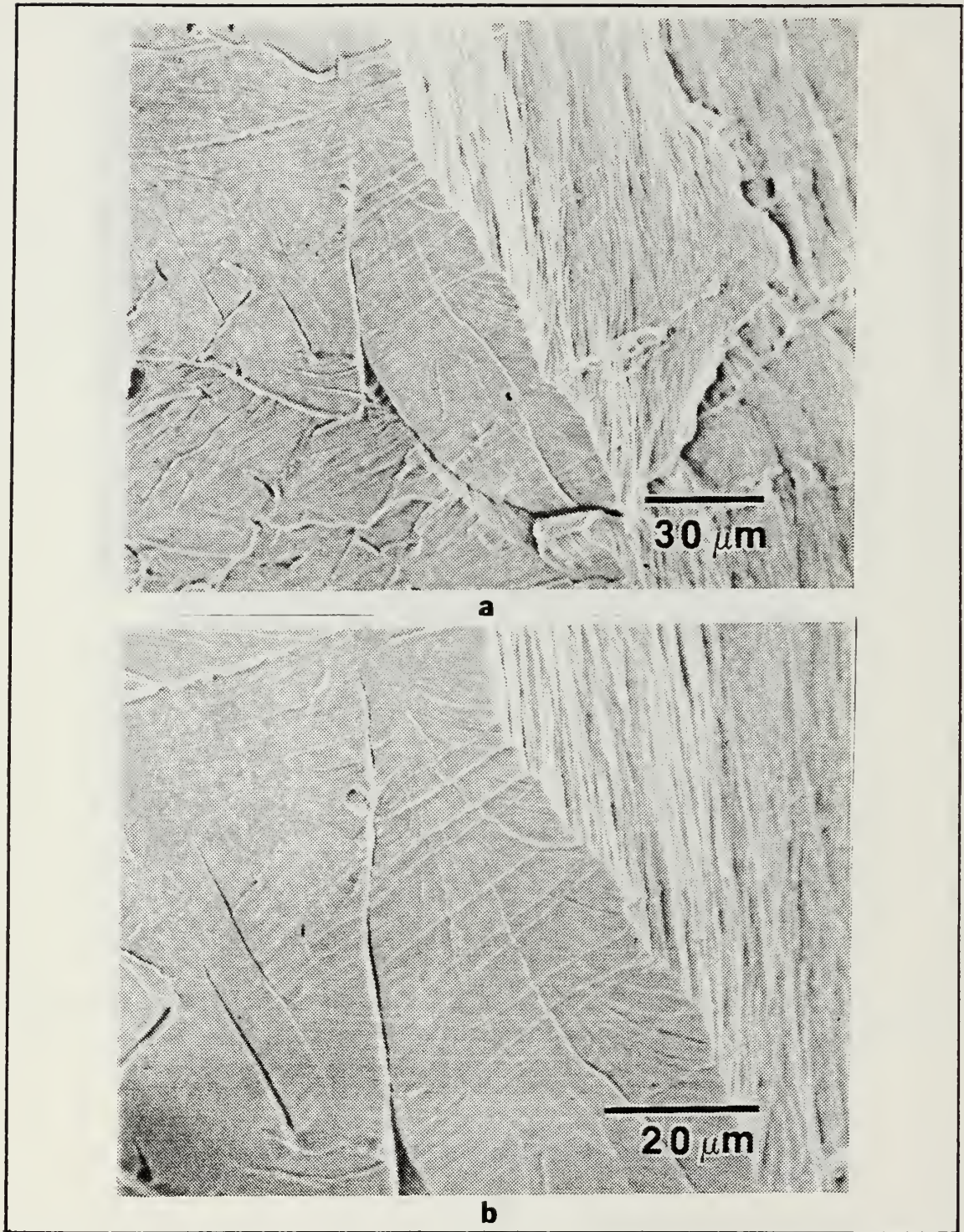
Figure A.5 Fracture Surface for Tensile Specimen of Furnace Cooled VACROSIL-010(Mo) annealed 1 hour at 900°C (a) 596X and (b) 1.15KX.
