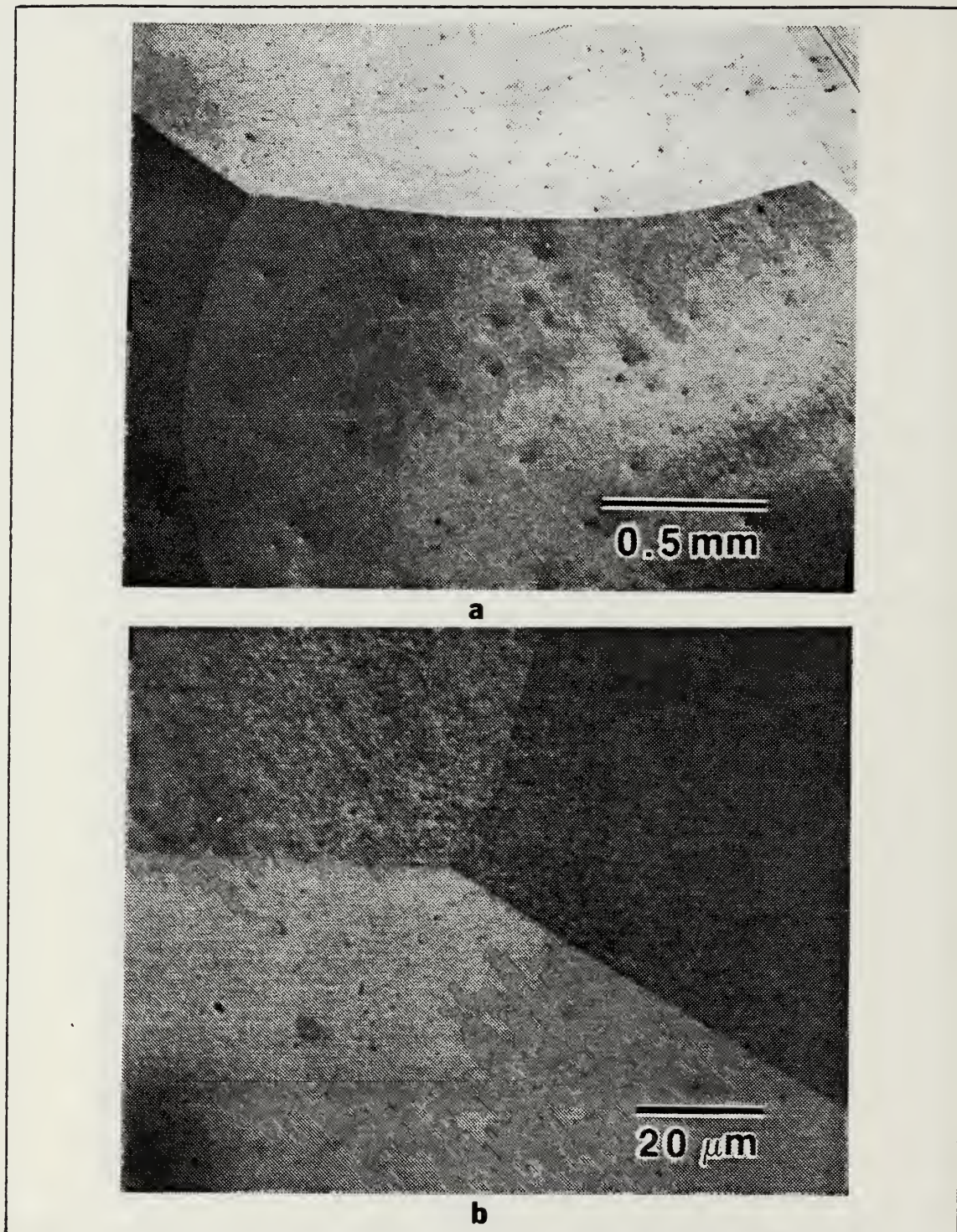
Figure 3.17 Optical Micrograph of Water Quenched VACROSIL-010(Mo) at (a) 50X and (b) 1000X Annealed 1 Hour at 1000°C.
