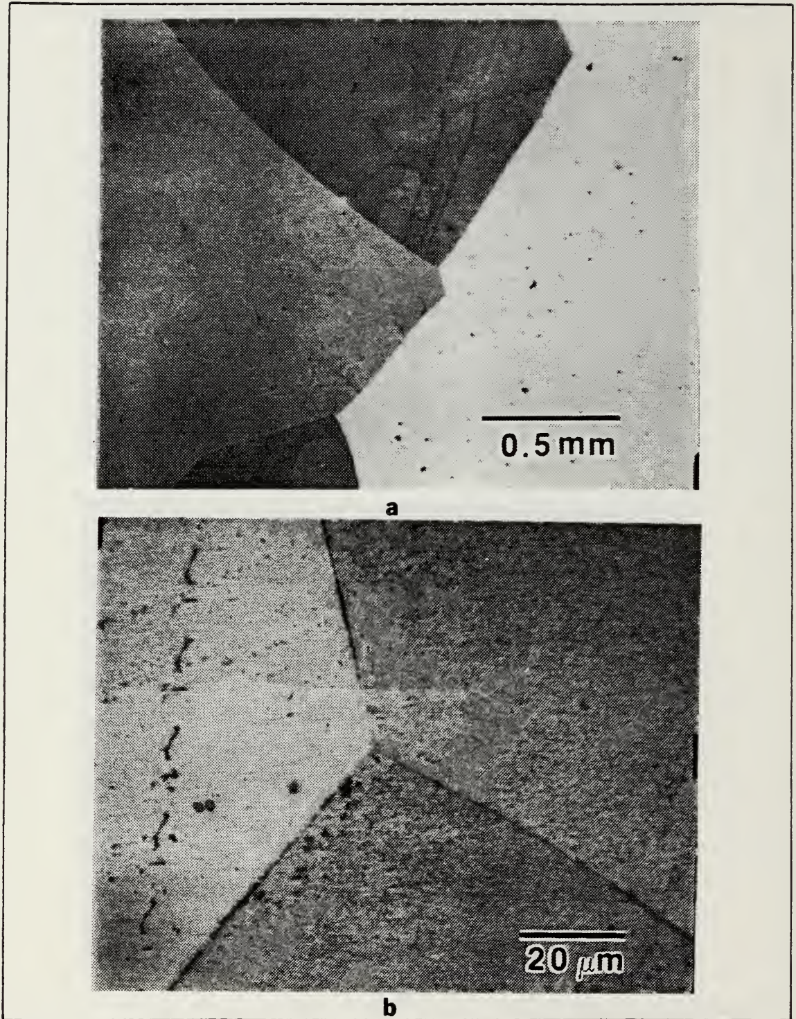
Figure 3.13 Optical Micrograph of Furnace Cooled VACROSIL-010(Mo) at (a) 50X and (b) 1000X Annealed 1 Hour at 1000°C.
