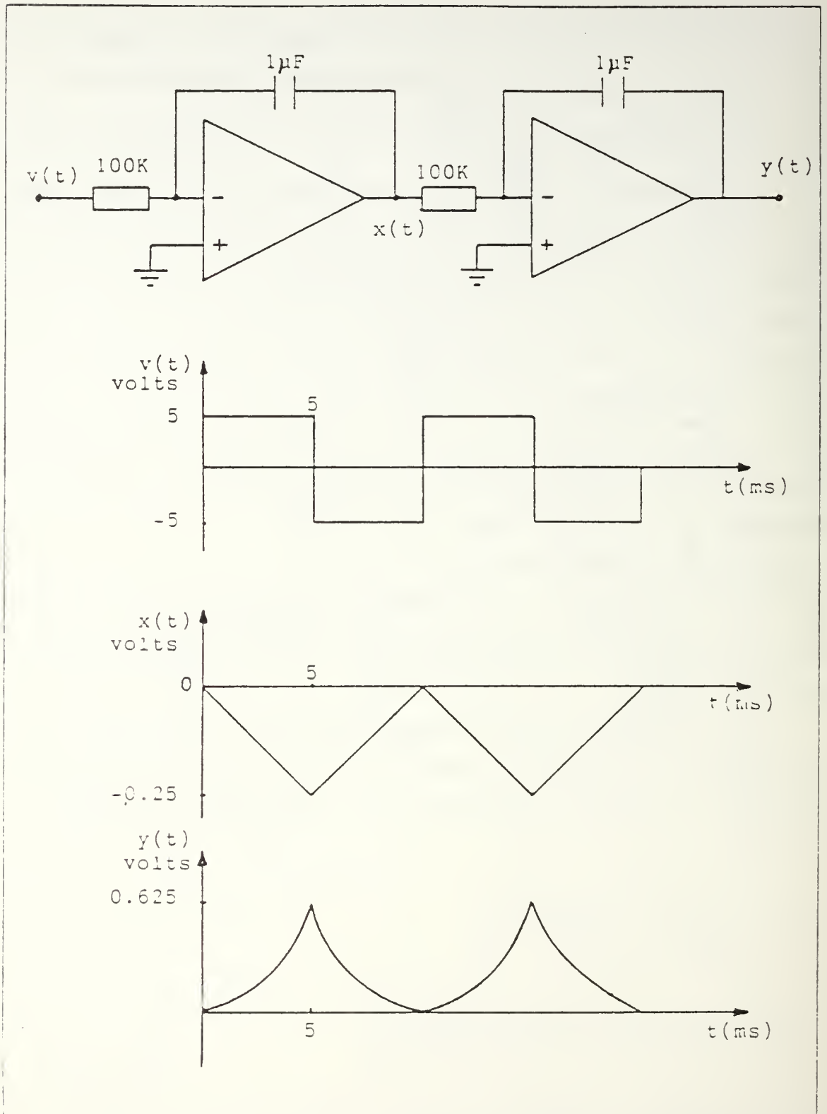
Figure 4.8 Double Integrator.
