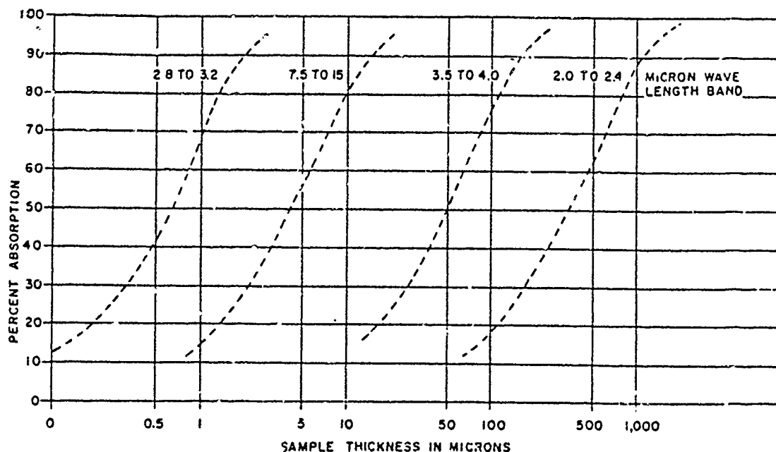
Figure 3.2 Sea water absorption for selected wavelength regions.
