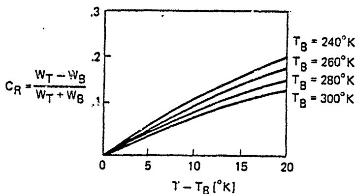
Figure 2.1 Radiation contrast for the 8-14 \mu\text{m} region.
