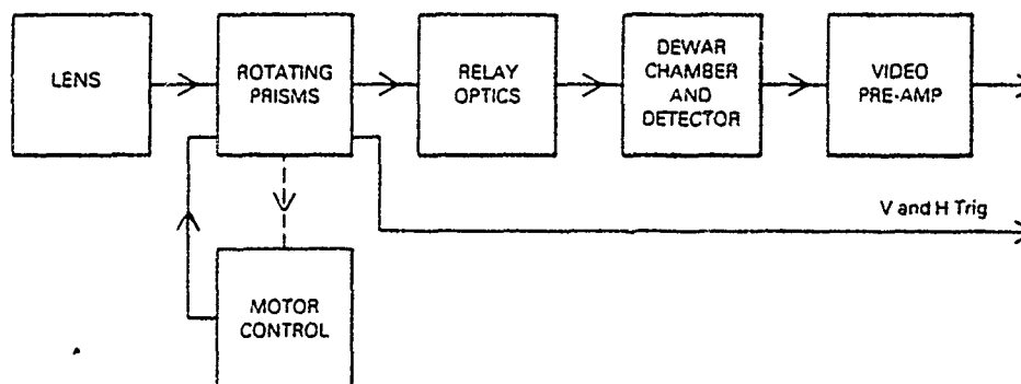
Figure 5.2 Simplified scanner unit block diagram.
