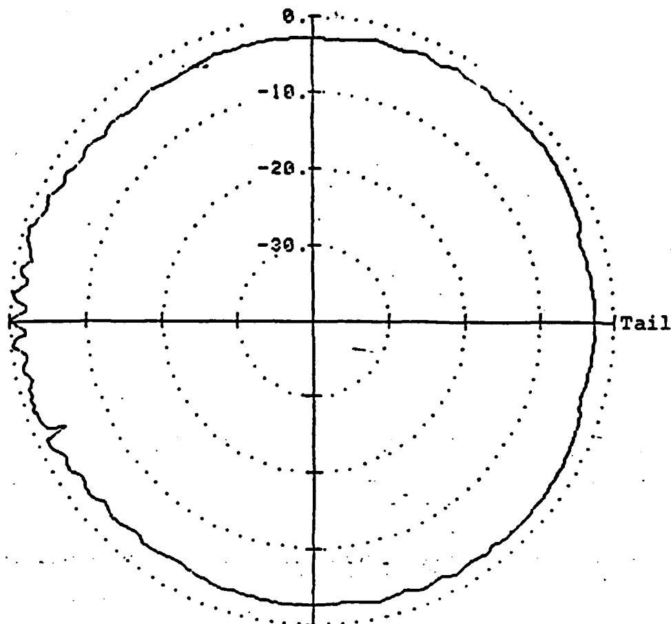
Azimuth Pattern (Antenna Station 316.3) Lower Rear Fuselage Landing Gear Deployed Elevation Angle Zero Degree Sikorsky S-76
