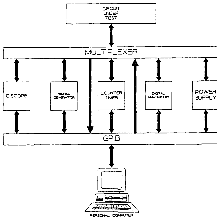
Figure 7.1 Proposed Student Work Station
