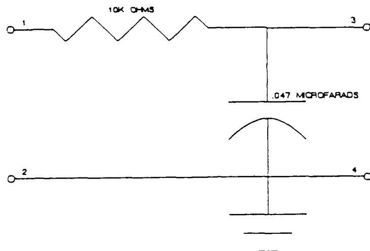
Figure 5.2 Low-Pass Filter
