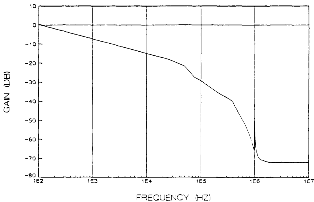
Figure 5.3 Bode Plot of the Low-Pass Filter Circuit
