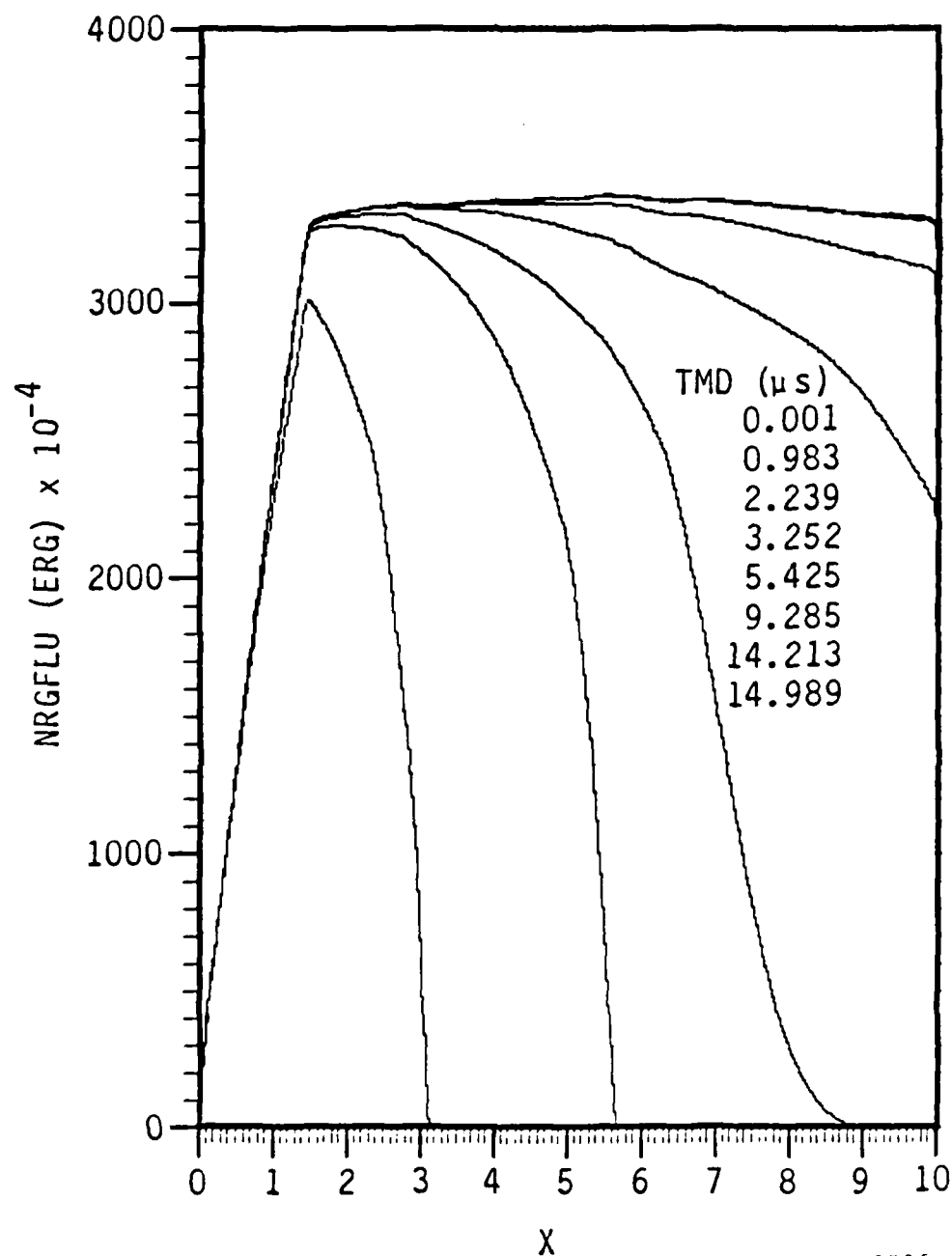
Figure 6. Total energy fluence profiles at various times. Hydrogen propellant. 0.54 g/s (10 atm) fill rate. 3.25J of laser energy deposited in 1.46 cm of nozzle gas. Nozzle filled for 20 \mu s (up to 5.6 cm).
