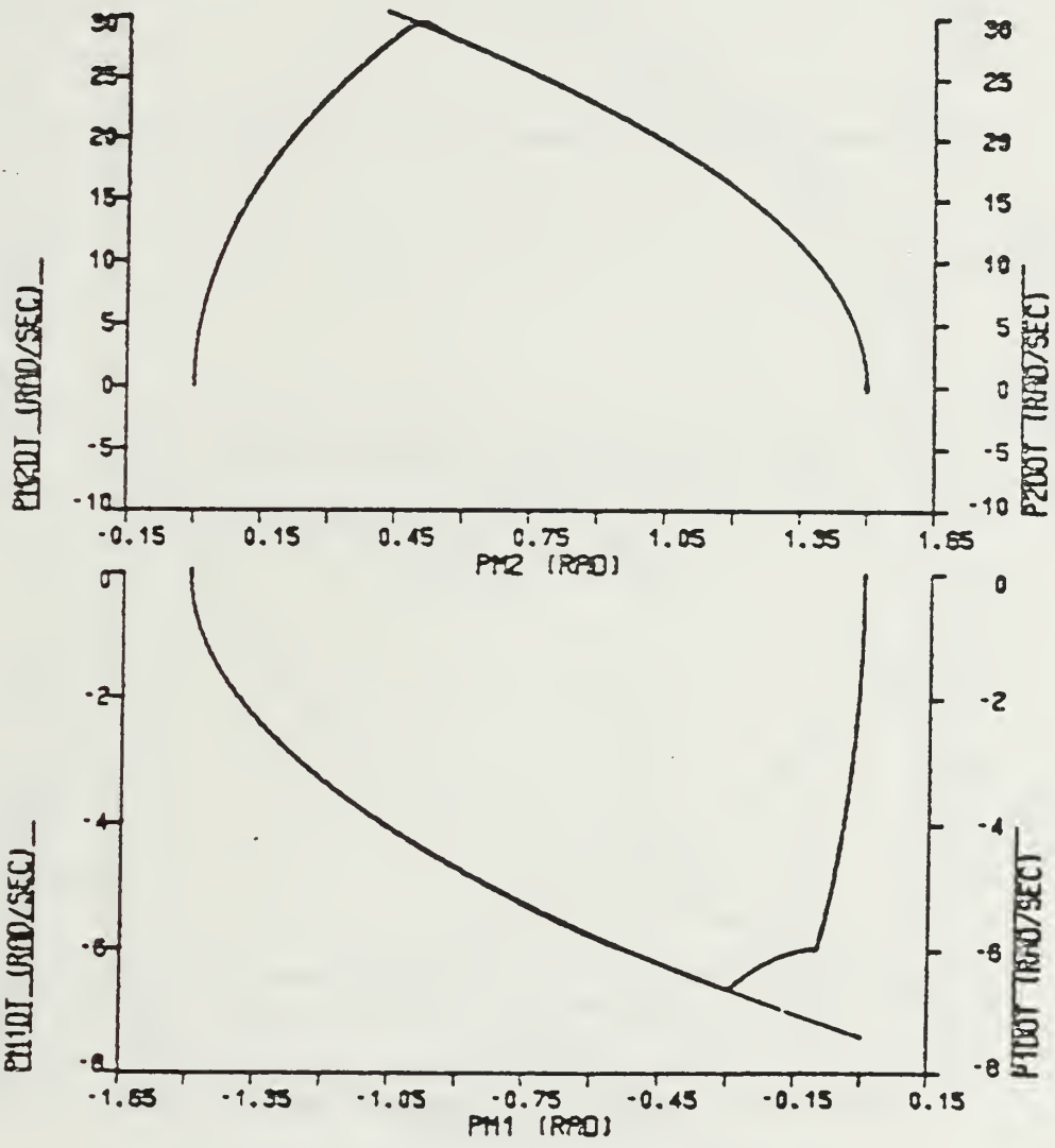
PHASE PLANE (CURRENT SOUR. DRV.)
