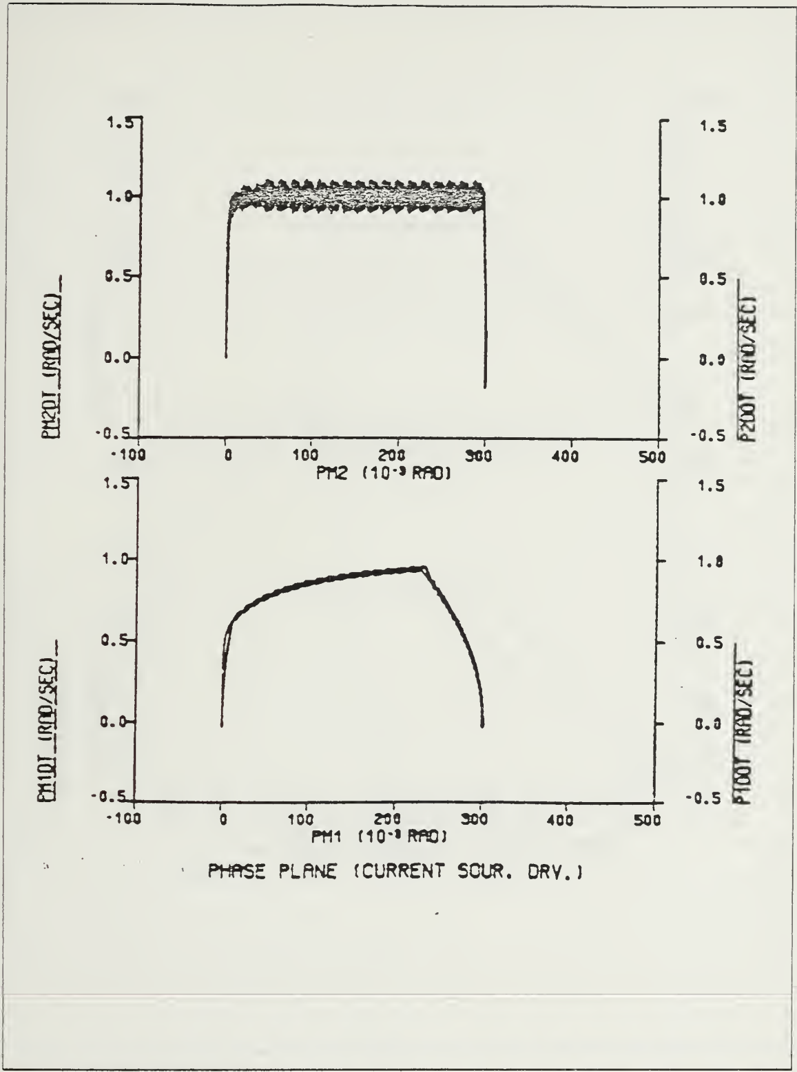
Figure 7.19 Phase Plane Trajectory For Ramp Input (No Gravity).
