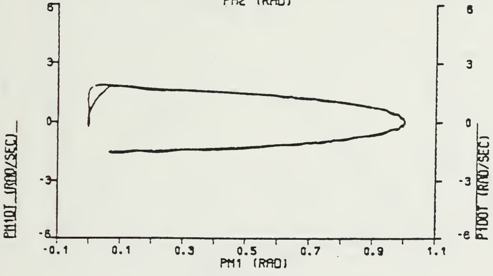
PHASE PLANE (VOLTAGE SOUR. DRV. WITH LOAD)
