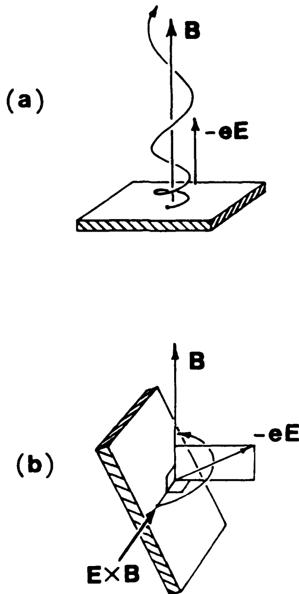
Figure 1. Effect of surface orientation on escape of emitted electrons. In (a), the spacecraft surface is perpendicular to the magnetic field B , and the emitted electrons, which experience an electric force -eE directed away from the surface, all escape. In (b), the spacecraft surface is nearly parallel to B , and almost all of the emitted electrons return to the surface, even though they still experience an electric force directed away from it. Note that the component of E perpendicular to B results only in an E \times B drift parallel to the surface.
