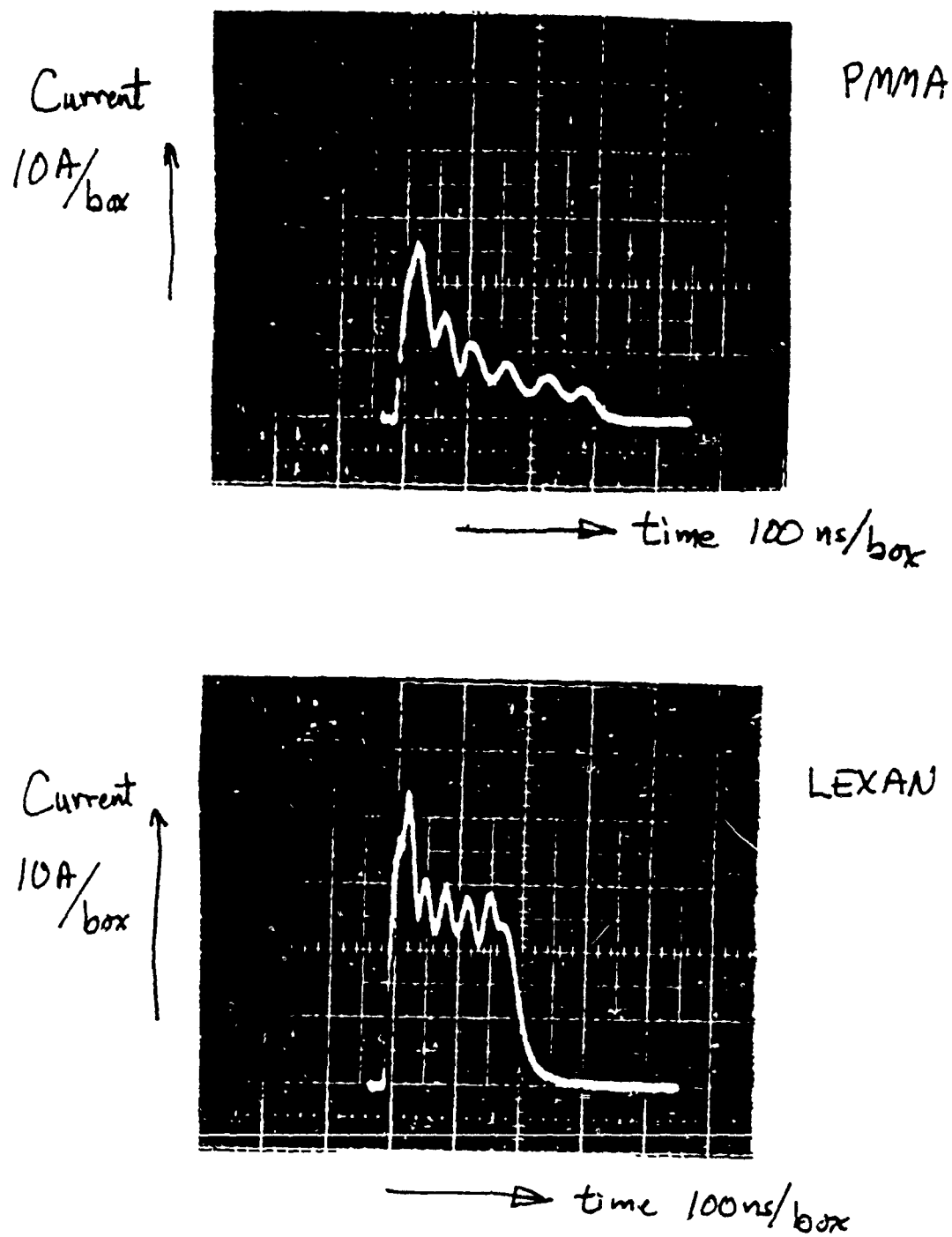
Figure 21 Channel Propagation vs Material 26 gap oscillating charge of 0.6\text{ }\mu\text{C}/\text{cm} , 2.5\text{ MeV}
