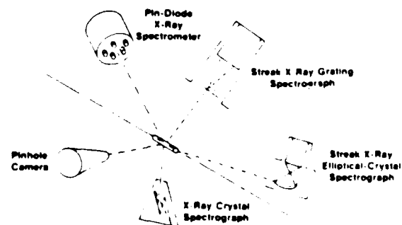
FIG. 6. Schematic of principal diagnostic systems deployed to characterize cylindrical plasma.
