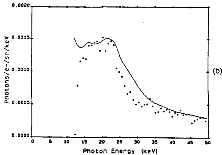
Ga 0.7 Al 0.3 As/GaAs (111) 16.9 MeV e- spectrum (Thickness = 8.8 microns)
