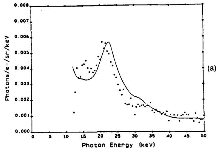
Ga 0.7 Al 0.3 As (111) 16.9 MeV e- spectrum (Thickness = 5.5 microns)
