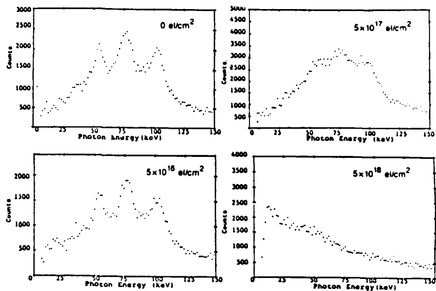
Figure 9: Channeling radiation from 54 MeV electrons channeled by (110) planes in LiF. The crystals were subjected to different dosages of electron beam irradiation: 0 \text{ electrons/cm}^2 , 5 \times 10^{16} \text{ electrons/cm}^2 , 5 \times 10^{17} \text{ electrons/cm}^2 , and 5 \times 10^{18} \text{ electrons/cm}^2 .
