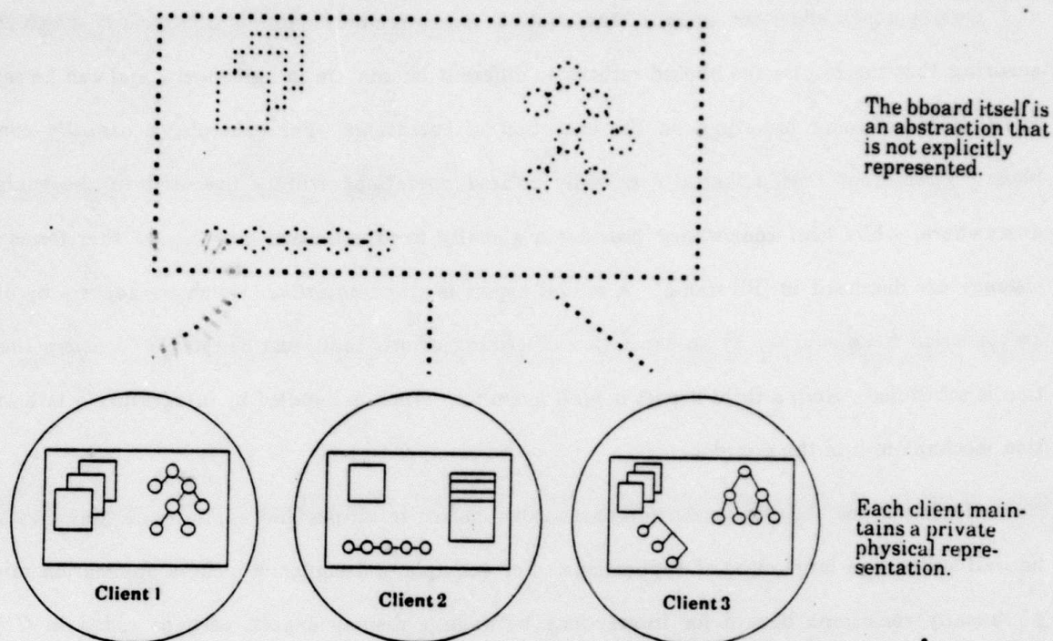
Figure 2: Clients interacting through a bboard
