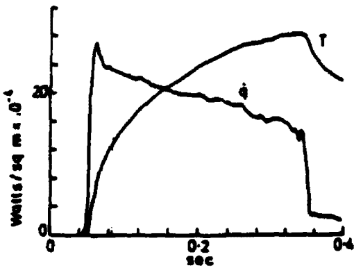
Variation of surface temperature T and heat transfer rate \dot{q} during run.
