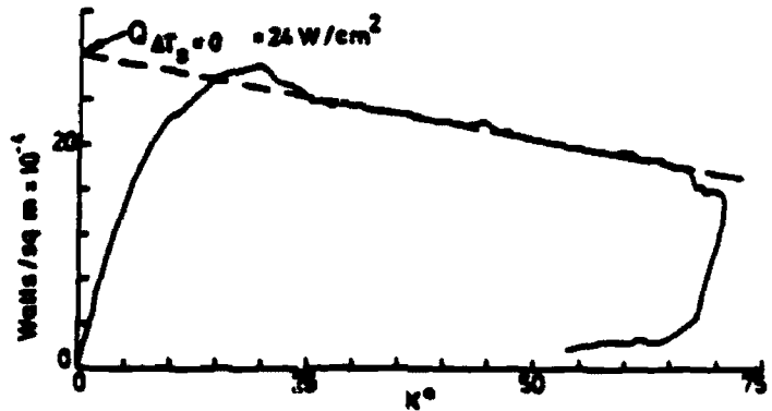
Heat transfer rate versus surface temperature.
