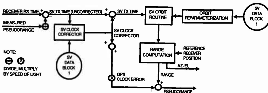
Figure 3. Pseudorange Computation
