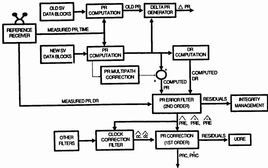
Figure 2. Pseudorange Correction Generation
