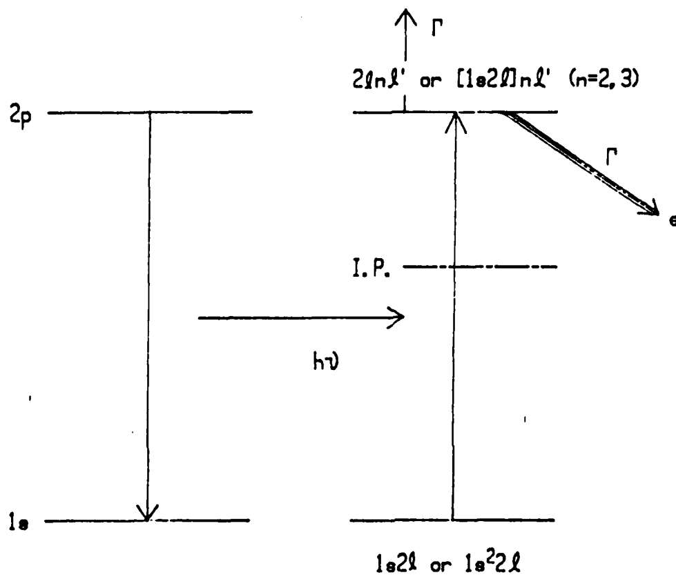
Fig. 1 — Energy level schematic for 2p - 1s matched-line pumping of helium-like 1s2l or lithium-like 1s^2 2l ground state to 2lnl' or [1s2l]nl' levels, respectively, above the ionization potential (I.P.). Rapid autoionization at a rate \Gamma dominates over radiative decay.
