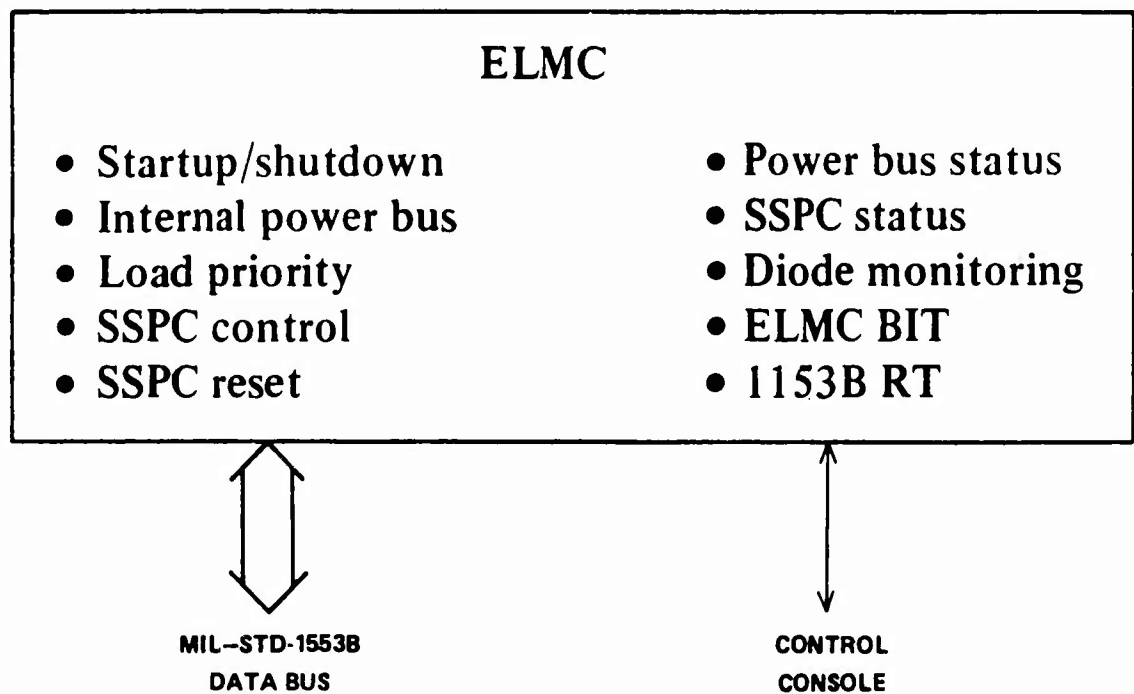
Figure 3.3-6. ELMC Functions
