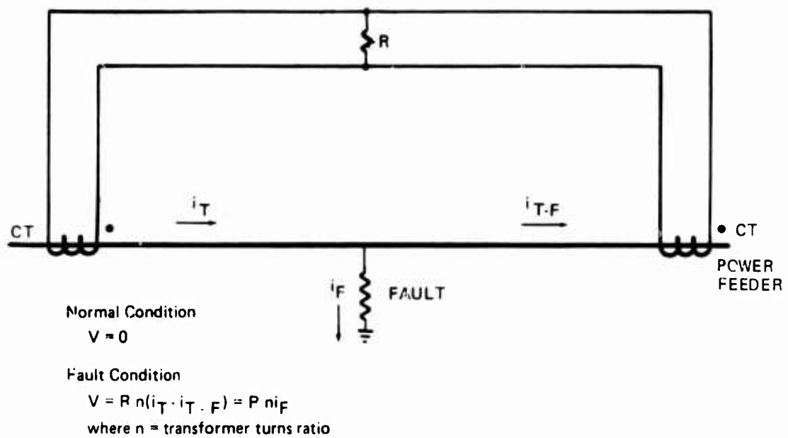
Figure 4.3.1-4. Differential Current Detection
