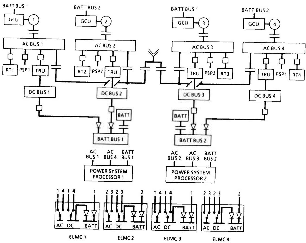
Figure 4.1.1-1. FTEPS Configuration
