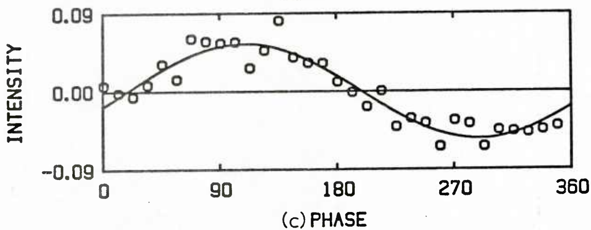
Figure 5.29 Phase averaged values at Re = 23,000 , f = 0.45 Hz, \omega^+ = 0.00495 and a = 0.098
