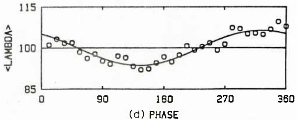
Figure 5.58 Phase averaged streak spacing at Re = 10,700 , f = 0.50 Hz, \omega^+ = 0.021 and a = 0.102
