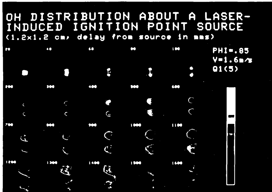
Fig. 1. Short-time sequence of planar OH distribution following deposition of laser energy at a point in a flowing \text{CH}_4 -air mixture. Times are in microseconds, beginning at 20 \mu\text{sec} after the pulse, and the region viewed is 1.2 x 1.2 cm.
