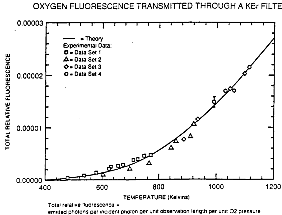
Fig. 3. Computed and measured O_2 fluorescence intensity versus temperature for excitation by a broadband argon fluoride laser.
