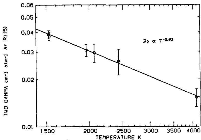
Fig. 4. Temperature dependence of the collision linewidth for Ar broadening; R_1(5) line at 0\text{H} . Best-fit temperature exponent is n = 0.93 .
