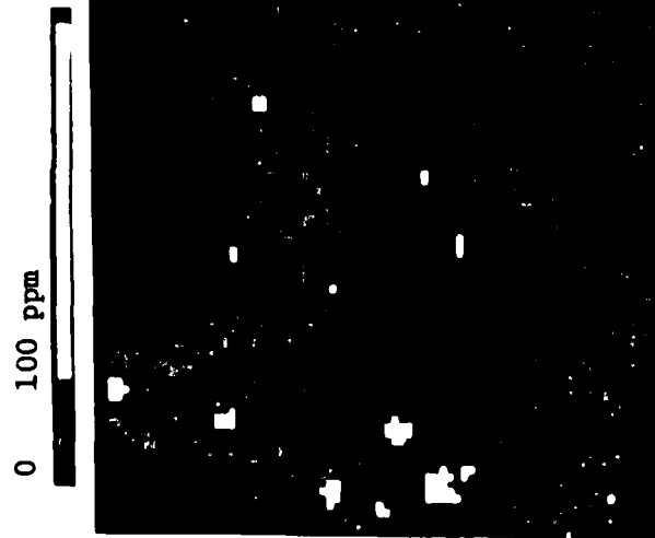
Digital Image of CH + Fuel Droplets in Heptane-Air Flame (1.2 cm x 1.2 cm)
