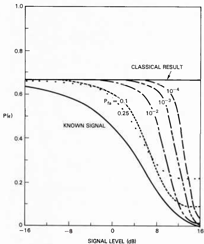
Fig. 12 — Error probabilities for Neyman-Pearson case, uncorrelated noise
