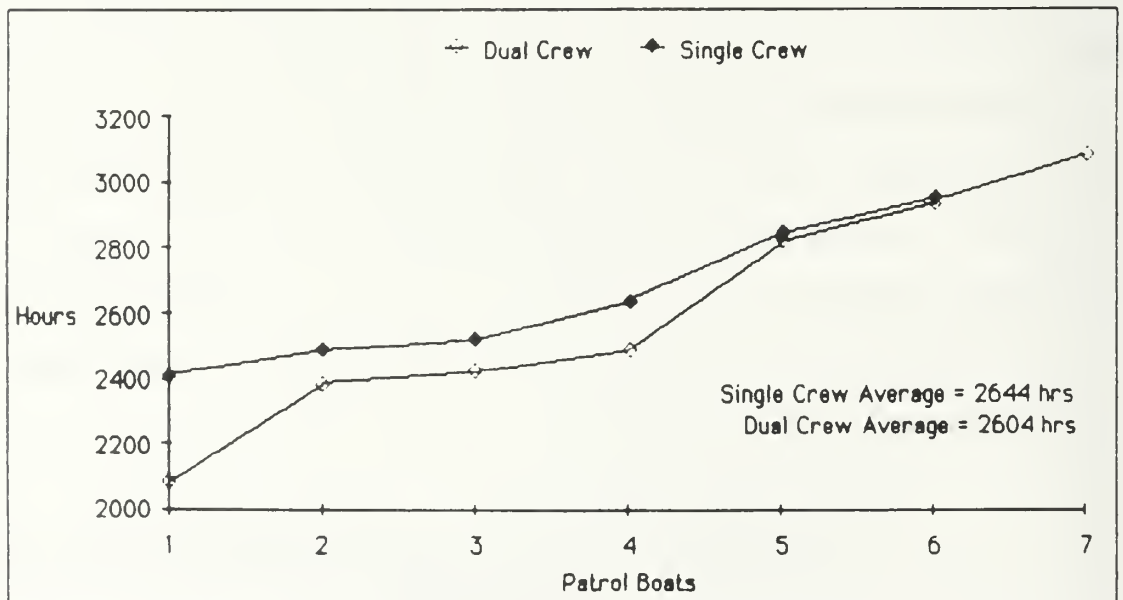
Figure 1. 82' WPB Maintenance Hours--FYs 84/85
