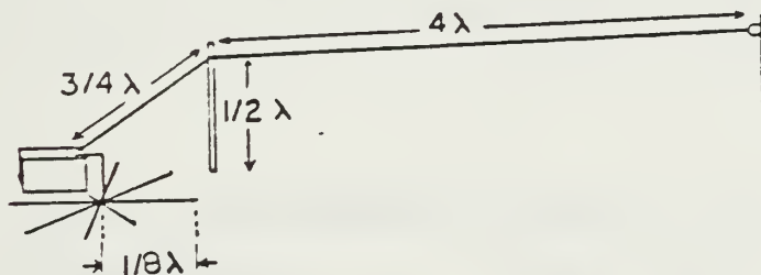
Figure 2.2 Antenna Configuration 1(d)
