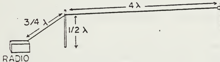
Figure 2.1 Antenna Configuration 1(a)
