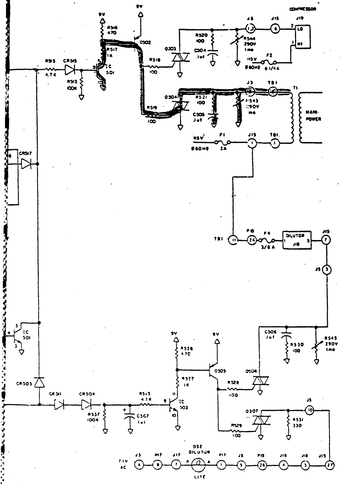
Figure 7.26 Flame Photometer Power Control Circuit
