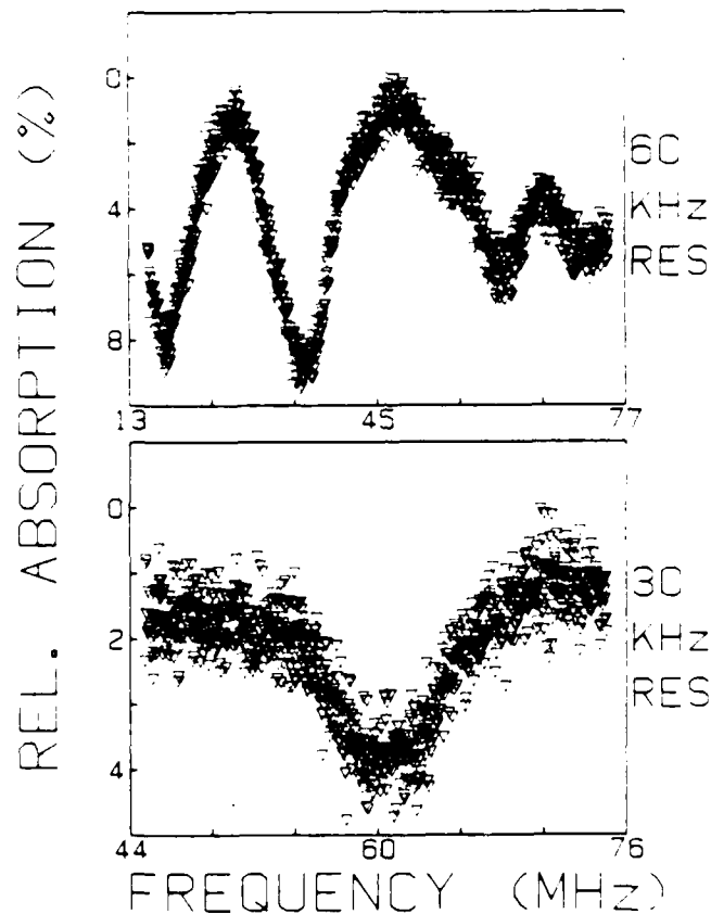
Figure 6 First continuously tuned FMS spectrum of a nuclear material, in this case the 14.4 keV transition of the simulation nucleus ^{57}\text{Fe} . Instrumental resolution is indicated and observed linewidths correspond to the transform of the lifetime of the nuclear state.
