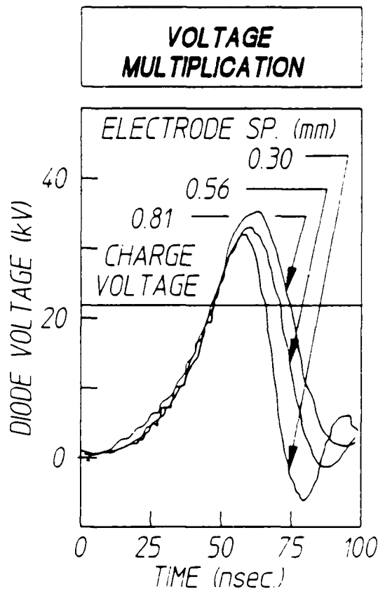
Figure 10: Voltages measured across the electrodes of the x-ray diode driven by system B as functions of time for the various spacings of anode to cathode indicated. Charge voltage of the Blumlein before commutation was 22 kV.
