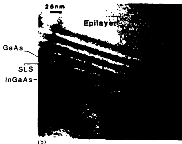
FIG. 3. TEM micrograph of GaAs-InGaAs superlattice. (a) Total thickness of the GaAs-In 0.14 Ga 0.86 As five-period SLS exceeds the critical thickness resulting in the generation of dislocations shown by arrows. (b) GaAs-In 0.06 Ga 0.94 As SLS composed of five periods of the 3000-Å "structures." Threading dislocations, shown by arrows, do not penetrate the SLS structure.
