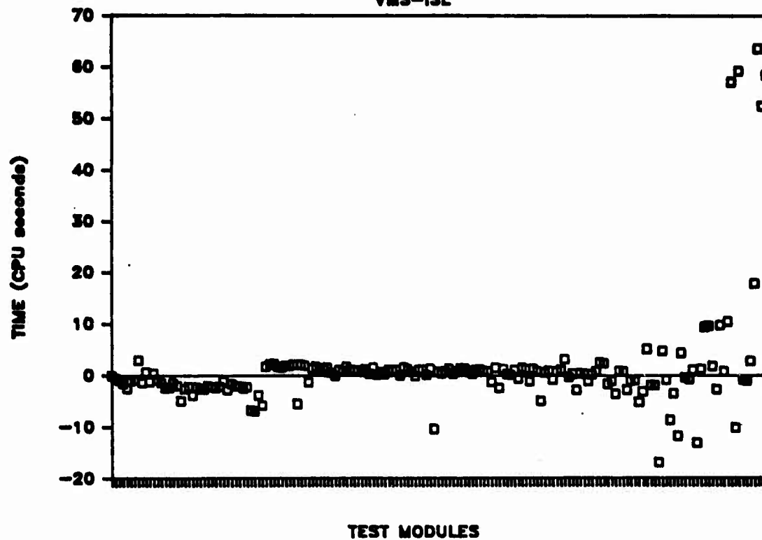
Fig. 4.5 VMS-ISL Compile Time: Actual vs Model Prediction
