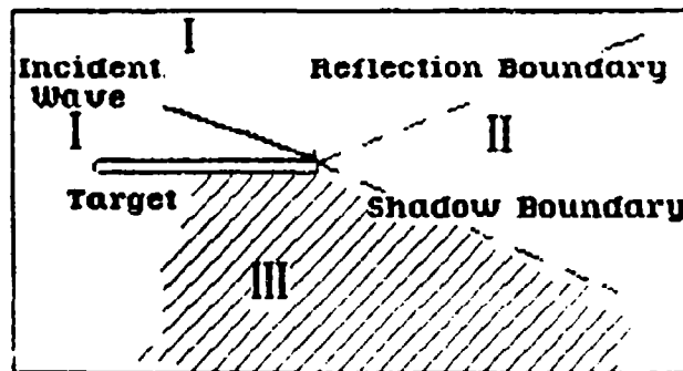
Fig 2.3. Diffraction Example.
