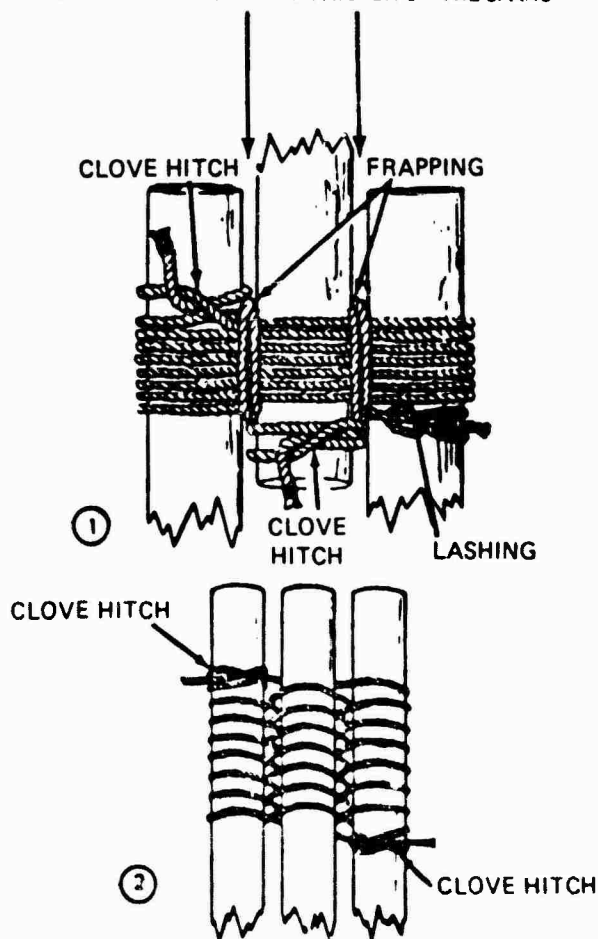
Figure 5-5. Lashing for a tripod
