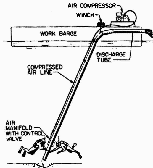
Figure 4-4. Airlift
