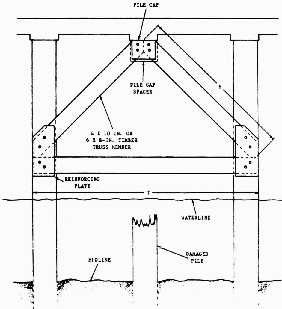
TIMBER TRUSS
