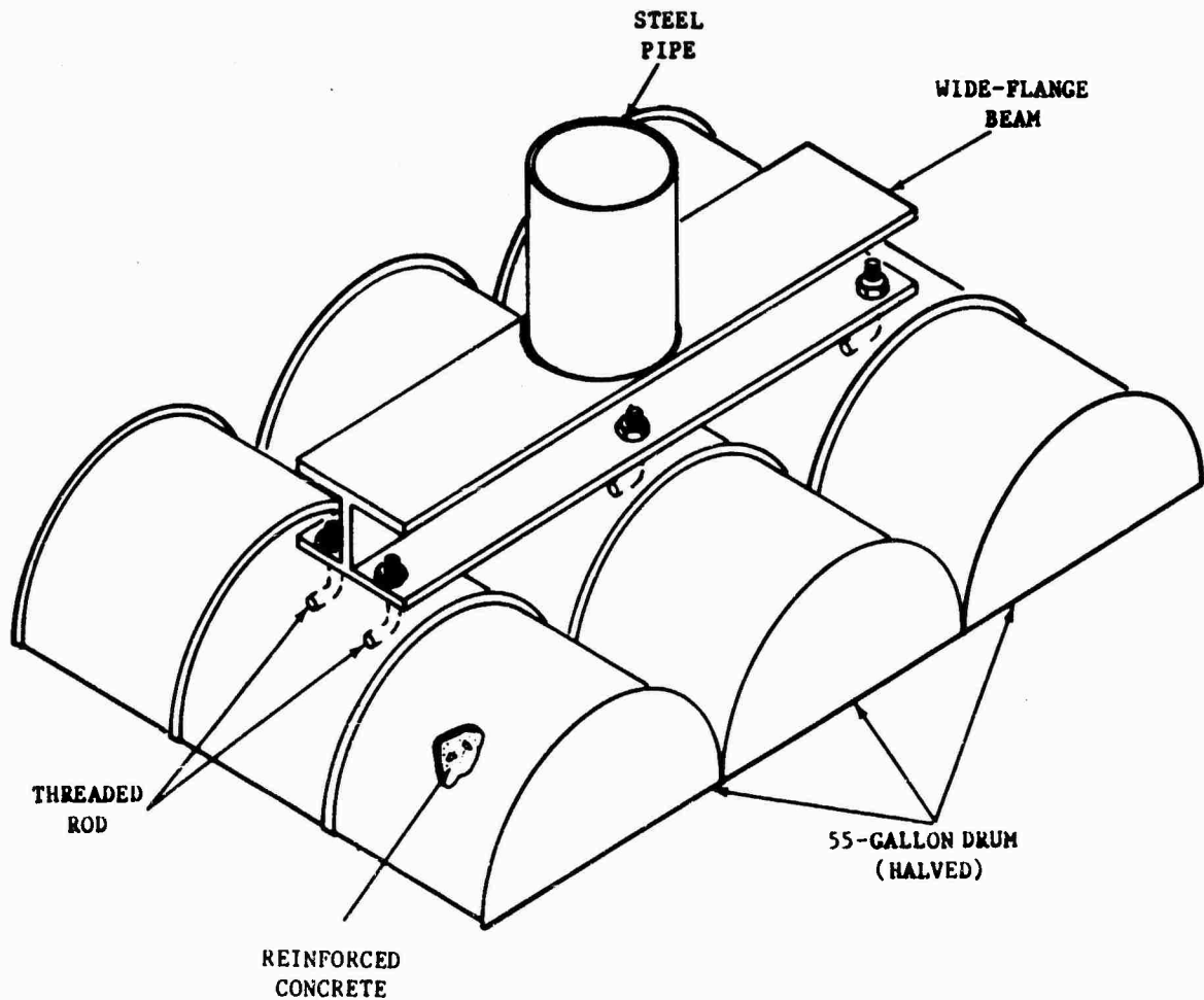
EXPEDIENT CONCRETE FOUNDATION
