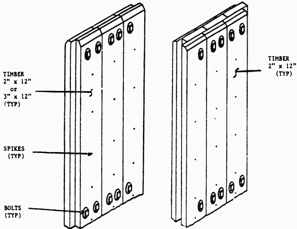
TIMBER SHEET PILING
