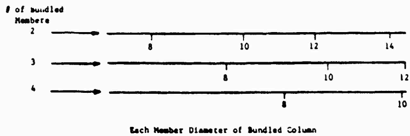
Figure 7-3. Replacement timber diameter determination
