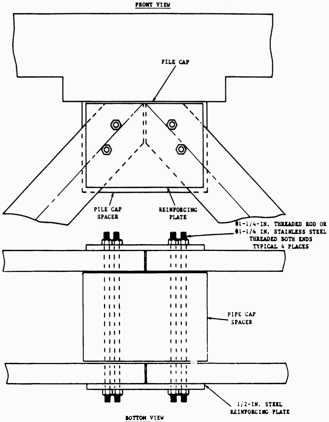
Figure 7-11. Timber truss pile cap connection
