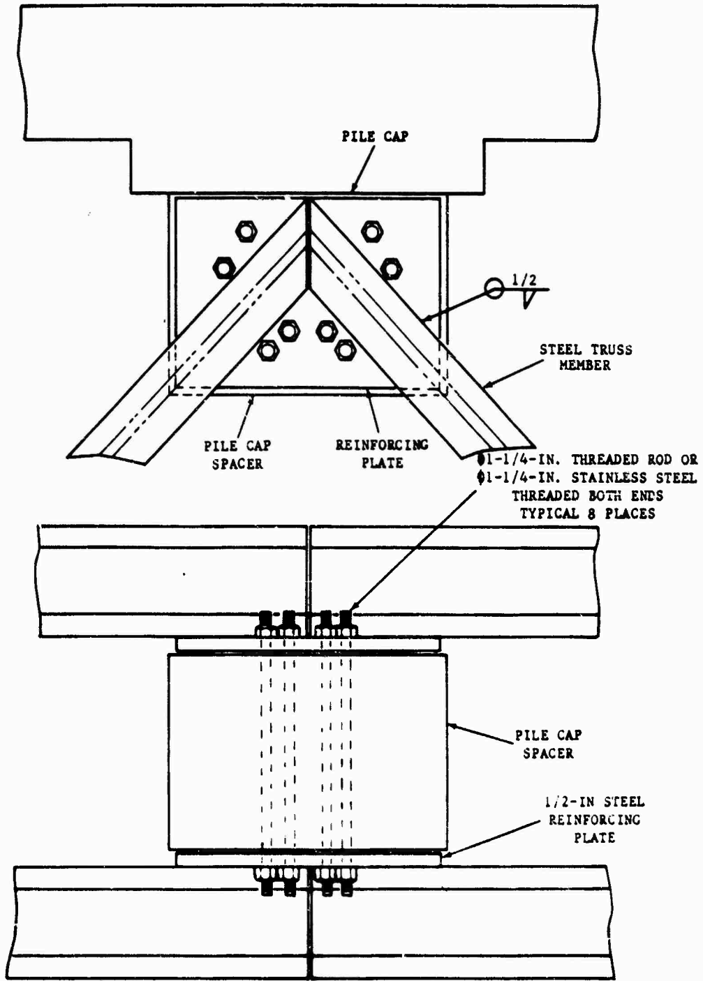
Figure 7-13. Steel truss pile cap connection
