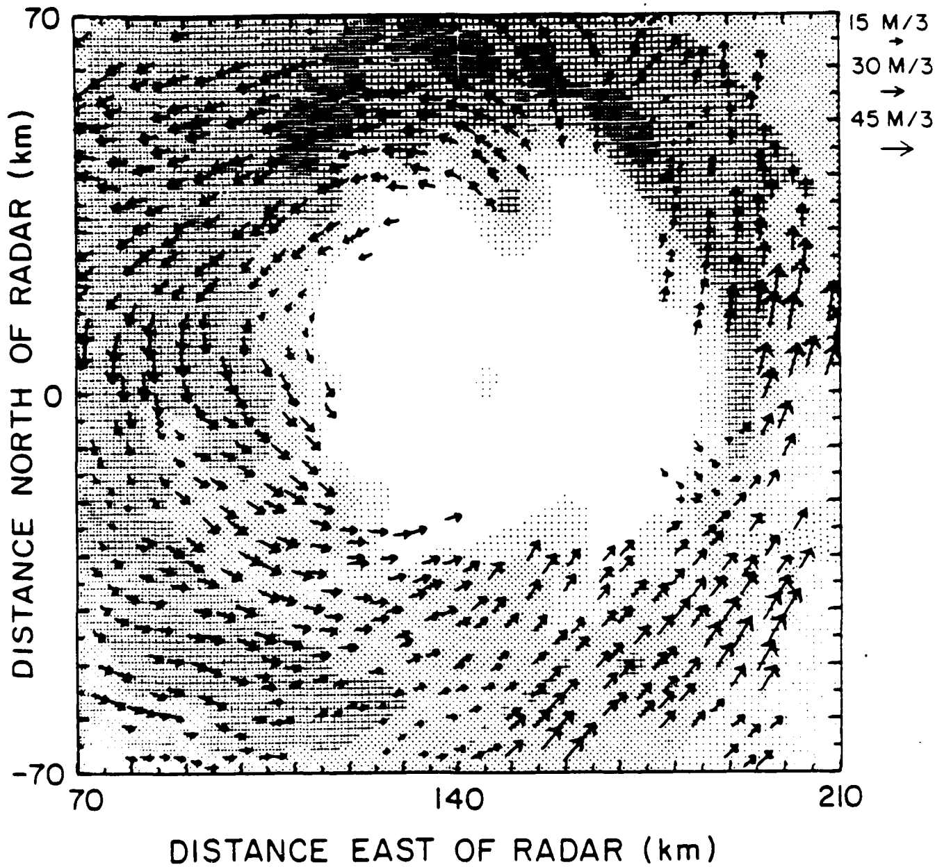
Figure 11. PPI of radar reflectivity data and TREC vectors for Hurricane FREDERIC collected by the Slidell, Louisiana NWS WSR-57 radar at 0331 UT on 12 September 1979 at 0.8 deg elevation. The shaded regions are reflectivity contours starting at 15 dBz and increasing at 10-dB interval (from Rinehart, 1982).
