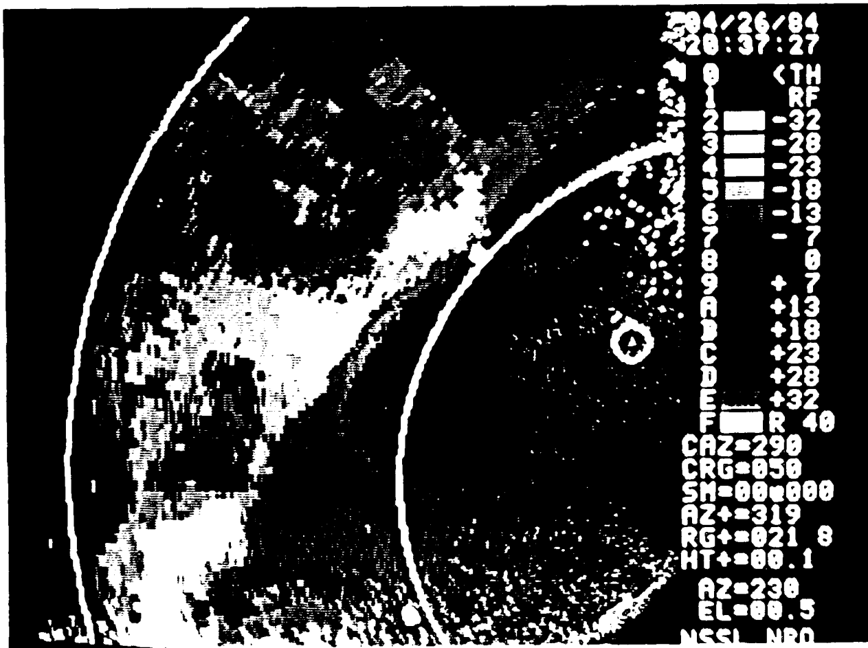
Figure 11: Example of radial velocity information obtained from meteorological doppler radar corresponding to the squall line in Figure 10. Negative velocities are toward the radar and positive velocities are away. A velocity differential of 60 m/s can be seen to the northwest with a squall line. Photo courtesy of the National Severe Storm Storm Prediction Center.
