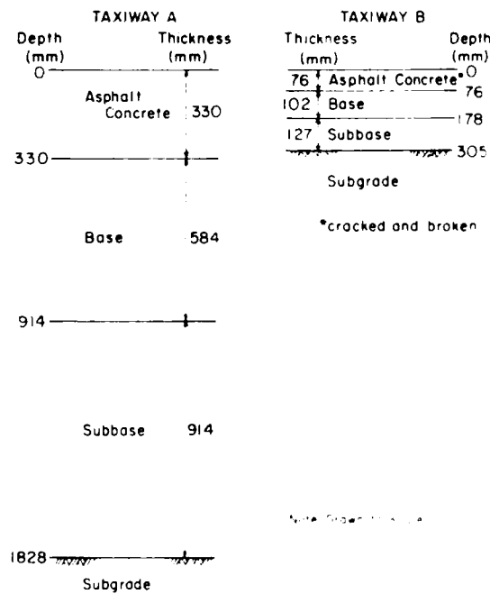
Figure 7. Pavement sections, Taxiways A and B
