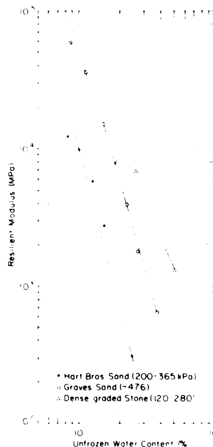
Figure 28. Resilient modulus vs unfrozen water content for three frozen Winchendon soils tested at 69 kPa confining stress and the indicated ranges of deviator stresses.
