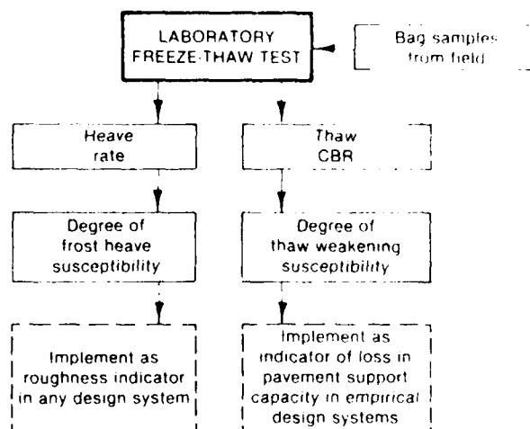
Figure 42. Implementation of the new freeze test.
