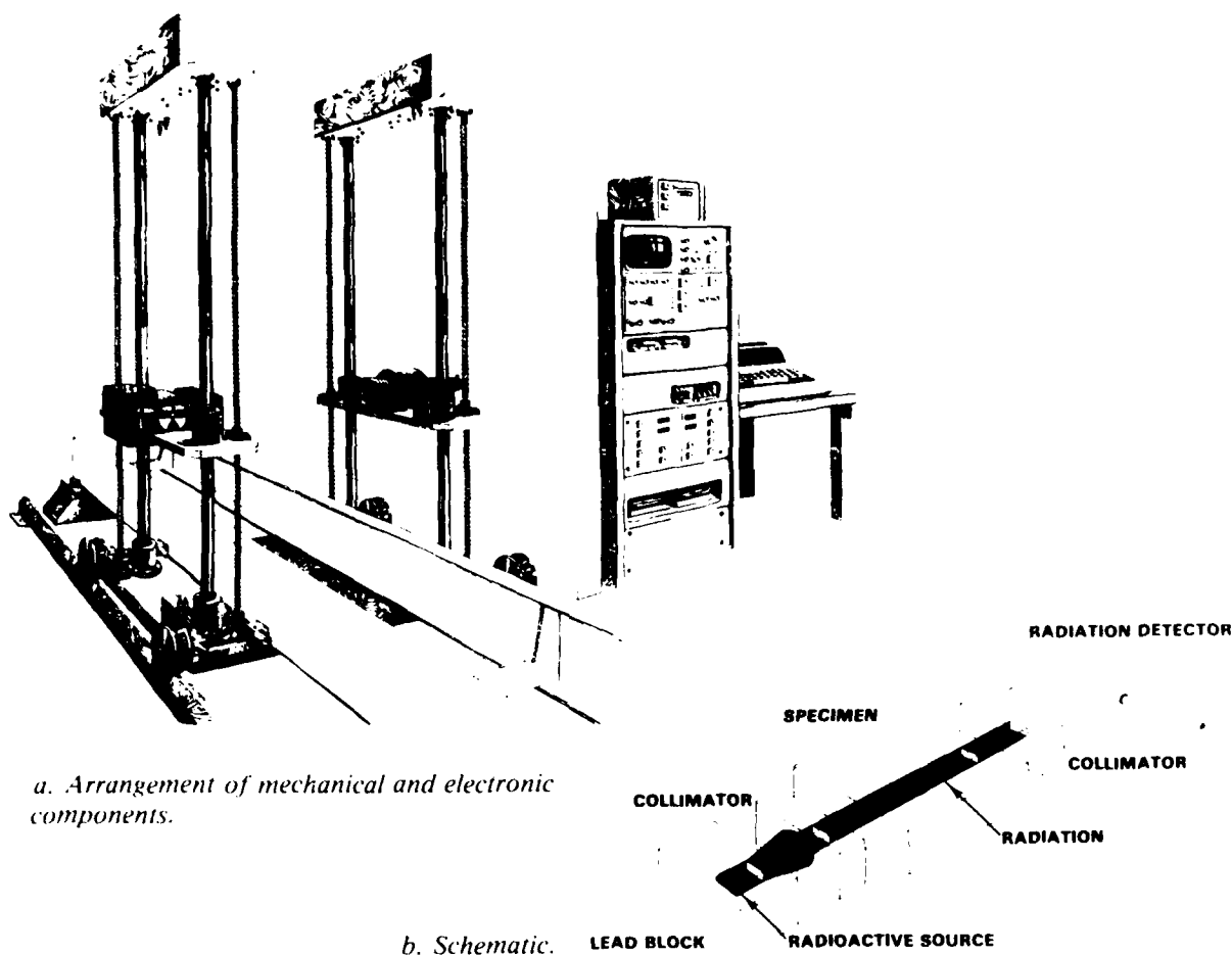
Figure 21. Dual gamma system.
