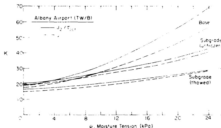
Figure 32. Coefficient K , of the empirical models (eq 9 and 10) vs moisture tension for several soils from Taxiway B, Albany Airport.
