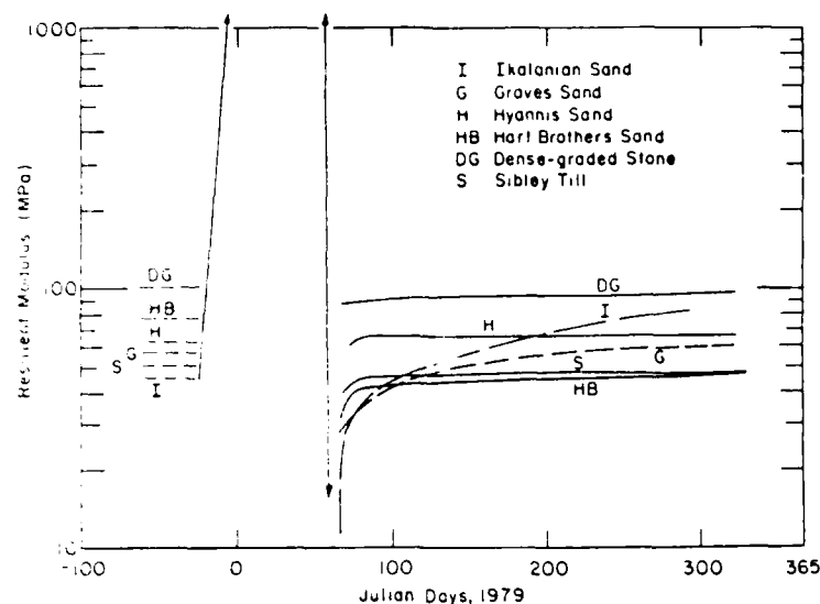
Figure 37. Interpretation of seasonal variation in the resilient modulus of six test soils directly beneath asphalt pavement under 200- to 300-kPa plate pressure.
