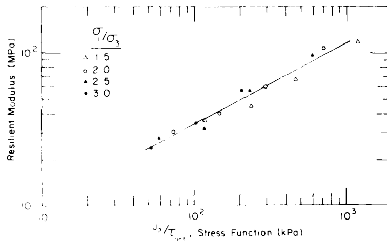
Figure 31. Resilient modulus vs J_2/\tau_{oct} for the test data given in Figure 30.
