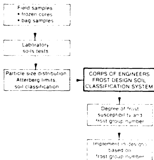
Figure 41. Implementation of the Corps of Engineers frost design soil classification system
