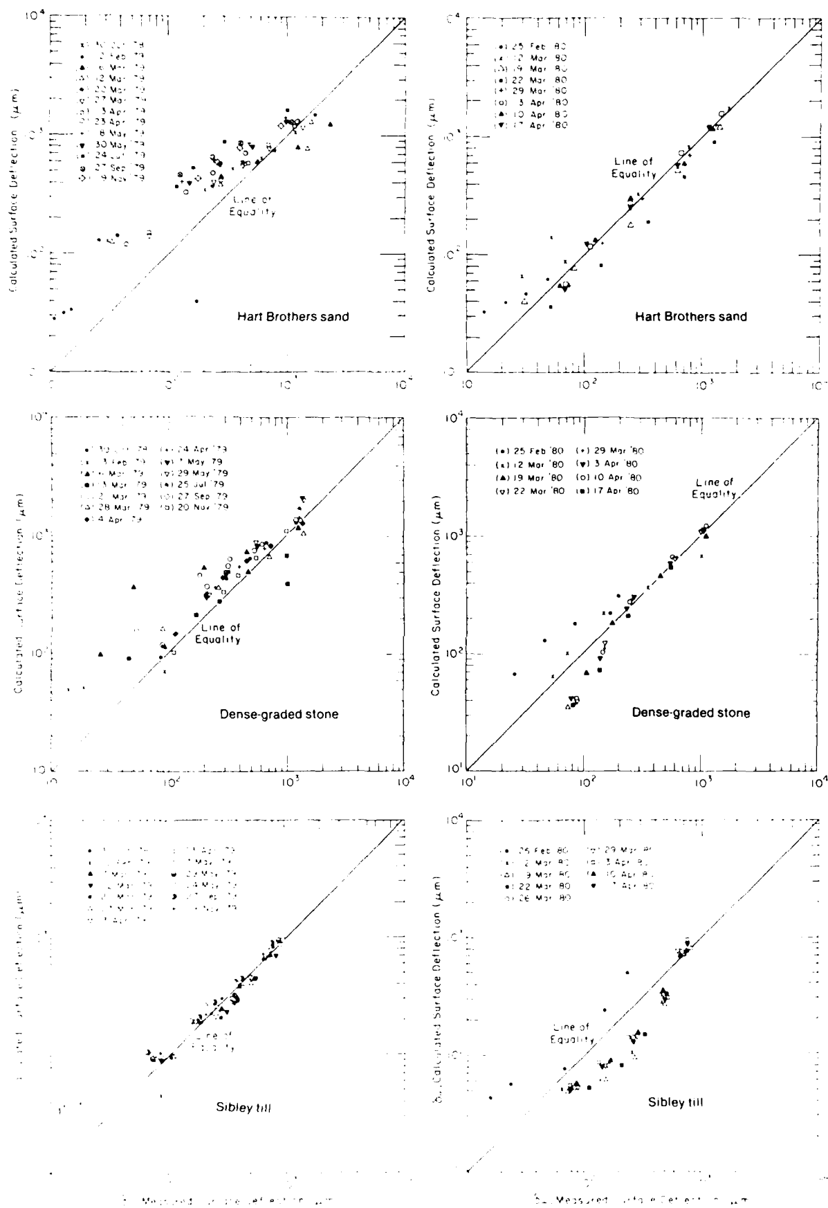
Figure 35. Measured surface deflections compared with deflections calculated by NELAPAV for three test sections.
