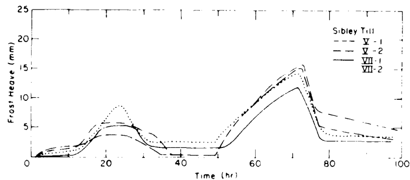
Figure 14. Frost-heave results for the new freeze-thaw test on four samples of Sibley till.
