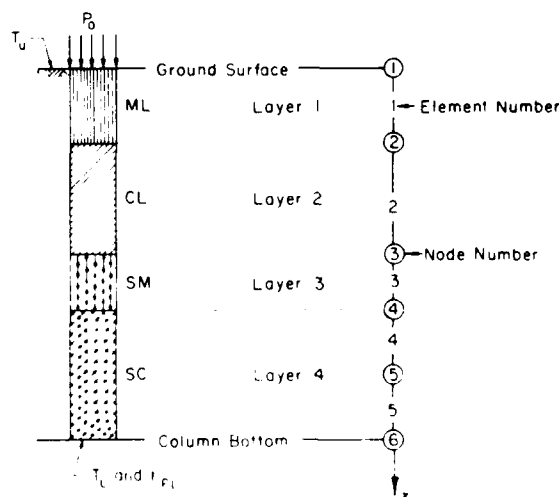
Figure 25. Nonuniform soil profile divided into elements and nodes and showing boundary conditions
