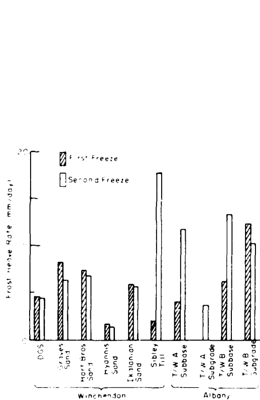
Figure 15. Heave rates for all test materials in new freeze-thaw test.
