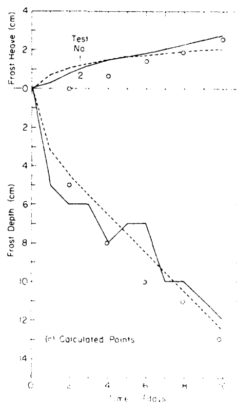
Figure 26. Measured and simulated frost depth and frost heave, laboratory soil-column test on Fairbanks silt.
