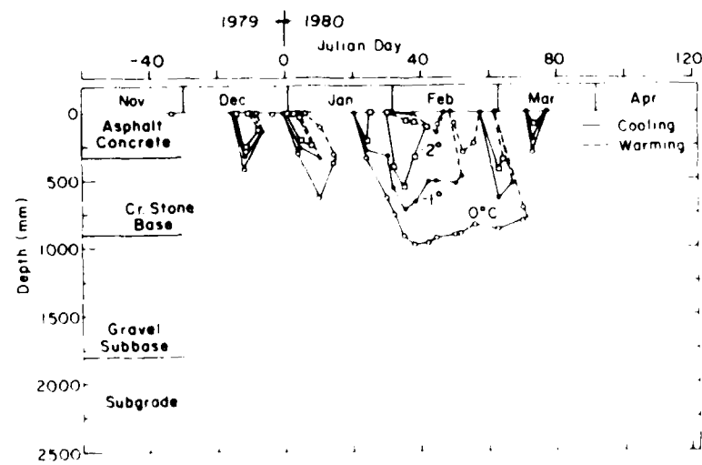
Figure 9. Freezing isotherms at Taxiway A, 1979-80.
