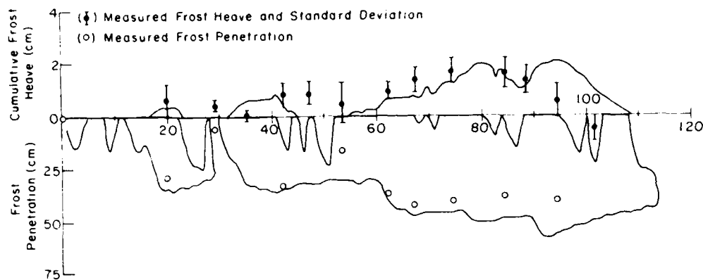
Figure 27. Measured and simulated frost depth and frost heave, Taxiway B, Albany County Airport, 1979-80.
