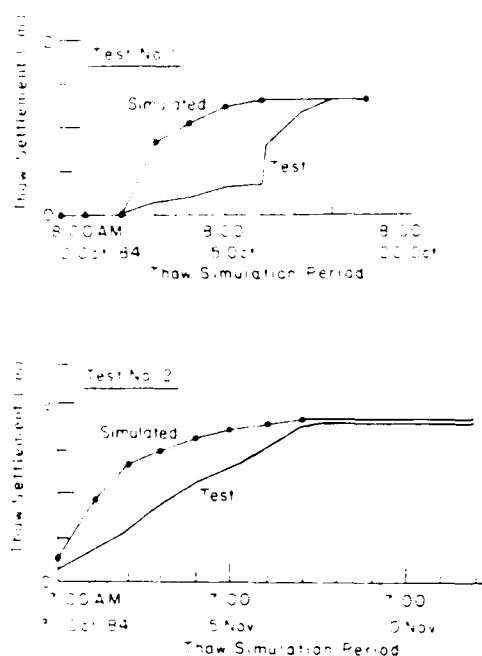
Figure 22. Thaw settlement in two soil-column tests on Graves sand.
