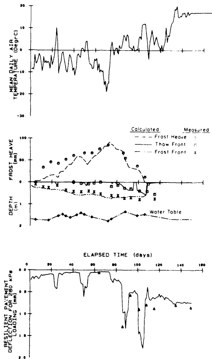
Figure 40. Comparison of simulated frost heave, frost and thaw depths, and pavement deflection with field observations, Graves sand test section, 1978-79.
