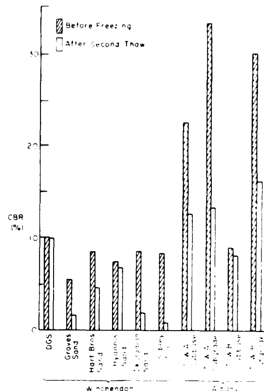
Figure 16. CBR values for all test materials in new freeze-thaw test.
