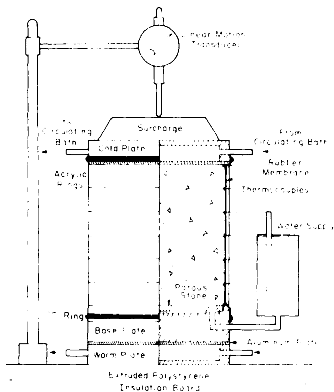
Figure 13. Schematic of new freezing test apparatus.
