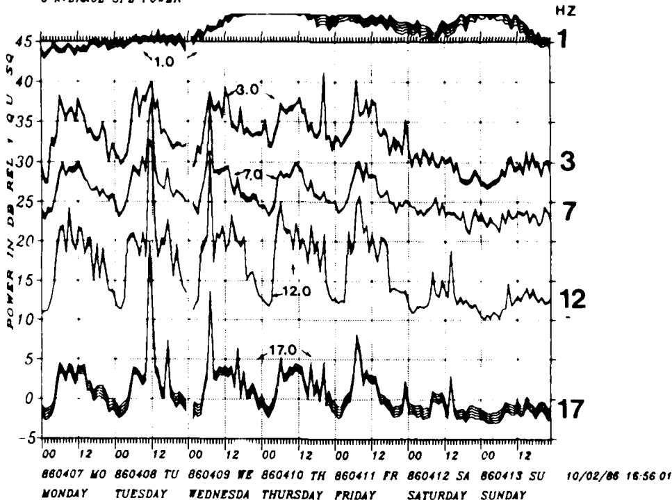
Fig. VII.7.1 Average NORESS SPZ spectral levels plotted on an hourly basis for a one-week period (week 15, 1986). The plots show a sequence of narrow frequency bands (+/- 0.1 Hz around the indicated center frequency). For better legibility, the data are shown in two separate diagrams, (top and bottom) with 5 frequency bands in each.
