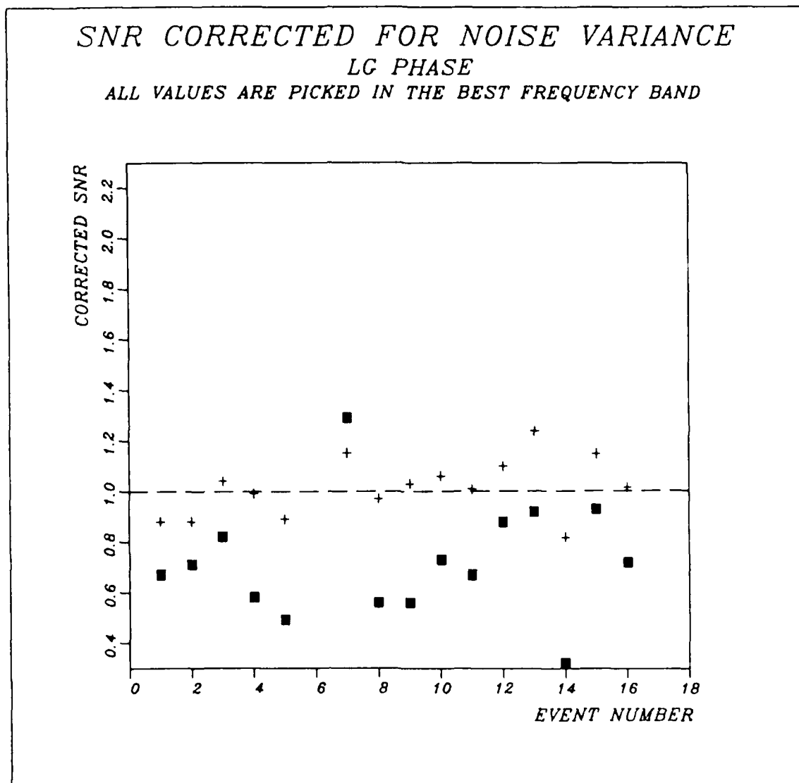
Fig. VII.3.4 Maximum corrected SNR relative to the corrected maximum of the AOZ, CRING and DRING configuration. The filled squares represent the beam of eight horizontal components. The crosses show the relative values of the beam with AOZ, CRING, DRING and the horizontal components, whereas the AOZ, CRING and DRING values are indicated by the dashed line at the 1.0 level.
