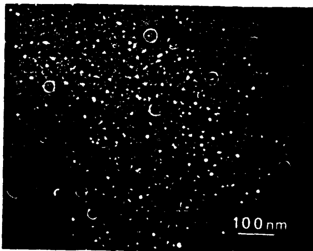
Fig. 2. Centered dark field image of Al-3%Li-0.12%Zr alloy aged at 150°C for 1000 min.
