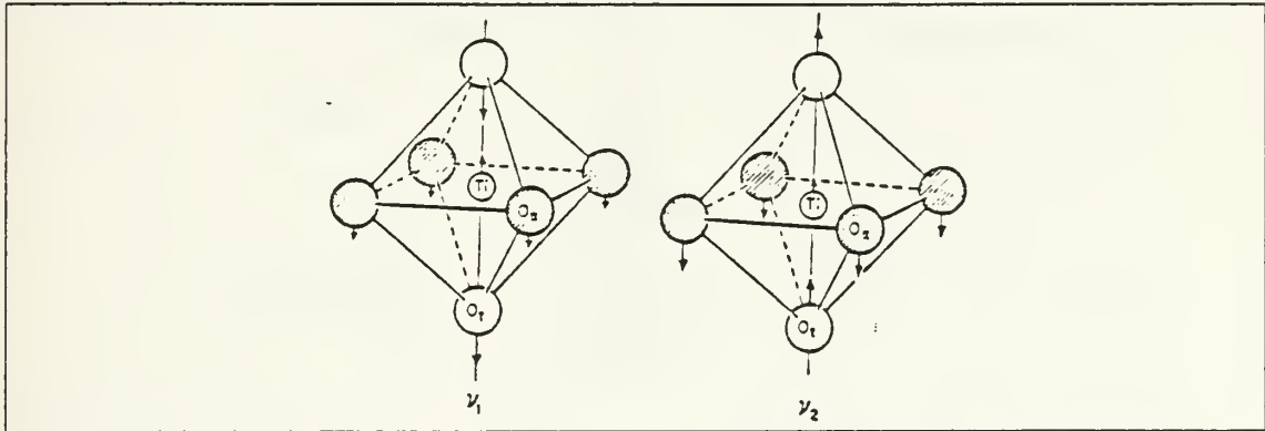
Figure 3.8 IR active normal vibrations of a TiO_6 octahedron [Ref.33].
