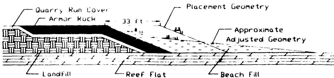
Figure 14. Revetment and beach-fill cross section
